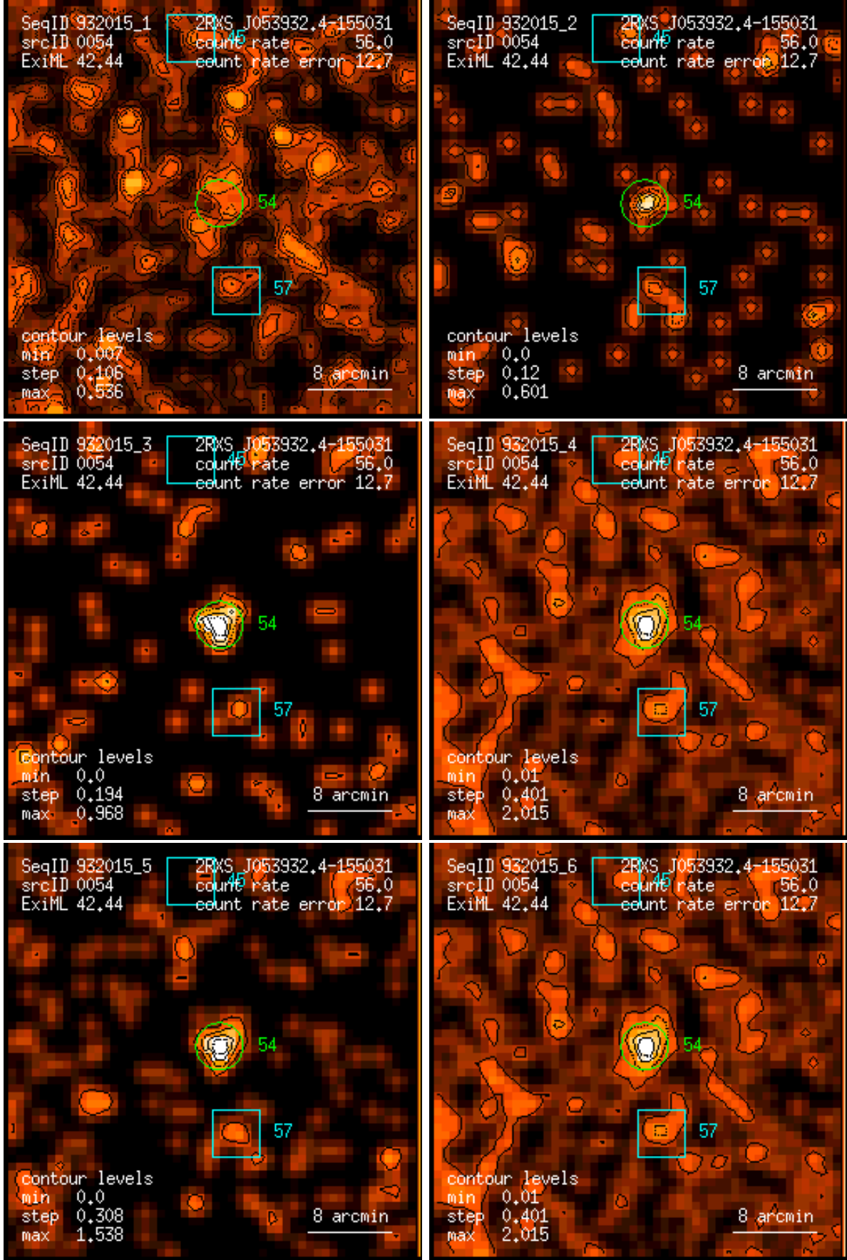
Figure 54: RASS 932015: detection 0054: band rate images, Gaussian filter: (1) PSPC channels 11 – 41, (2) 52 – 90, (3) 91 – 201, (4) 11 – 235, (5) 52 – 201, (6) 11 – 201. Broad band rates in counts/ks. Band rate contour levels in counts/ks/arcmin 2 .
