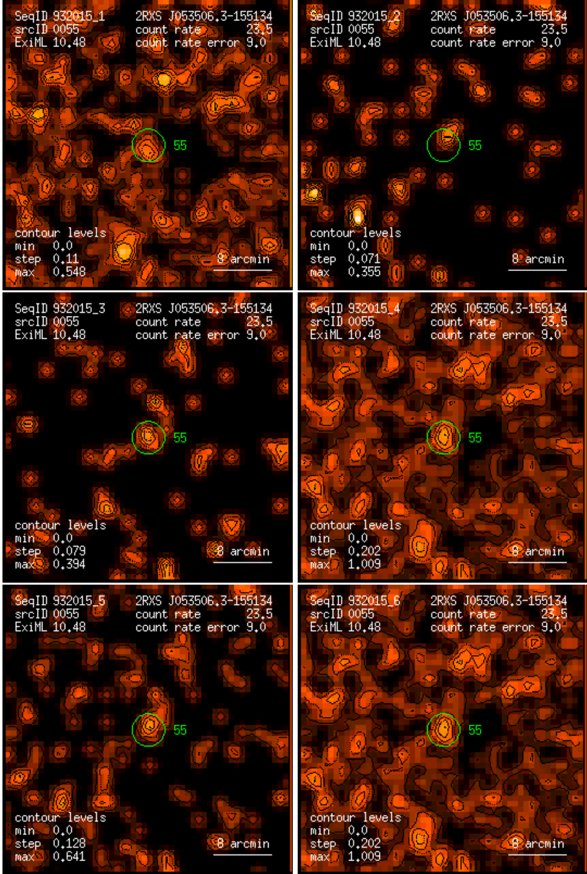
Figure 55: RASS 932015: detection 0055: band rate images, Gaussian filter: (1) PSPC channels 11 – 41, (2) 52 – 90, (3) 91 – 201, (4) 11 – 235, (5) 52 – 201, (6) 11 – 201. Broad band rates in counts/ks. Band rate contour levels in counts/ks/arcmin 2 .
