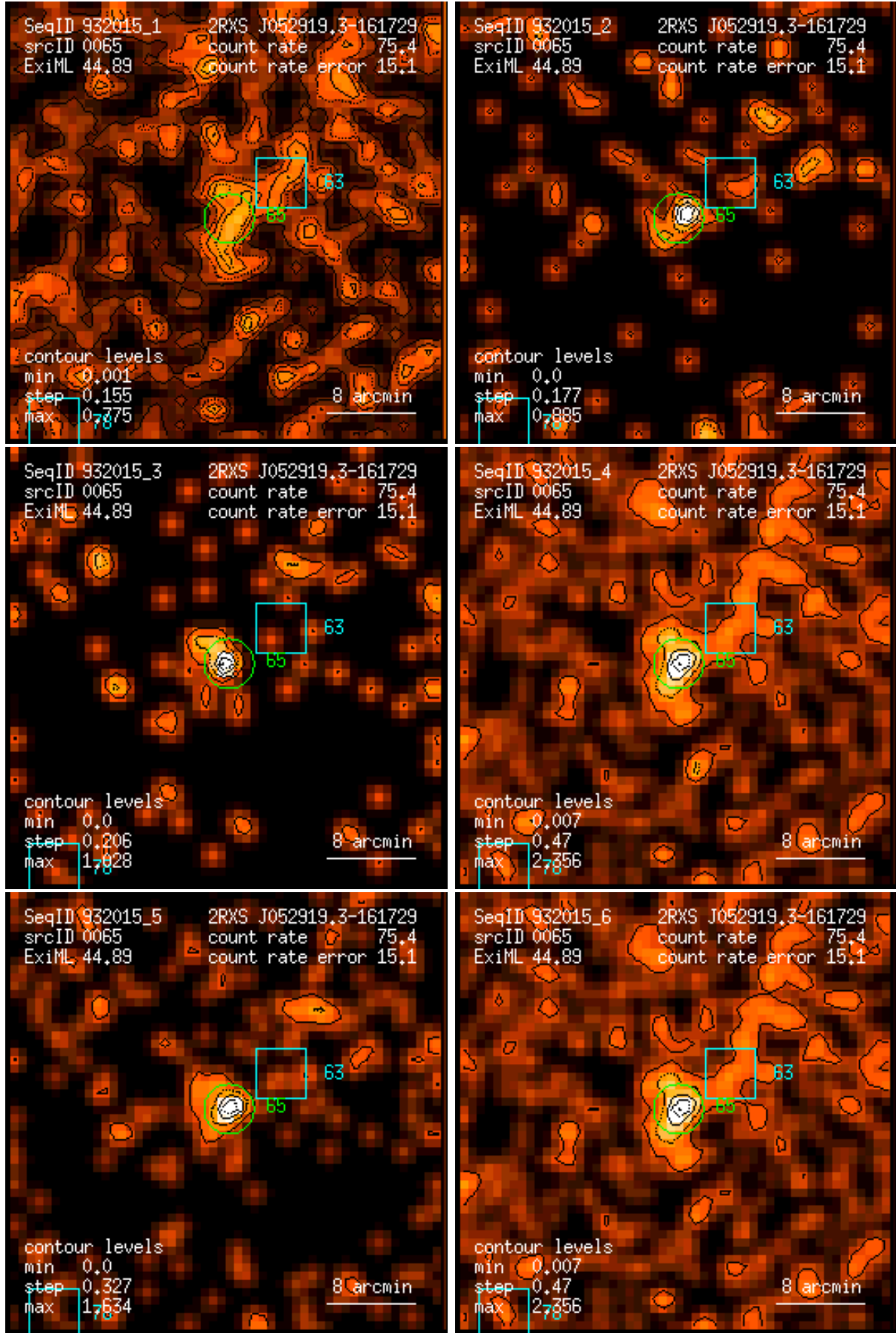
Figure 65: RASS 932015: detection 0065: band rate images, Gaussian filter: (1) PSPC channels 11 – 41, (2) 52 – 90, (3) 91 – 201, (4) 11 – 235, (5) 52 – 201, (6) 11 – 201. Broad band rates in counts/ks. Band rate contour levels in counts/ks/arcmin 2 .
