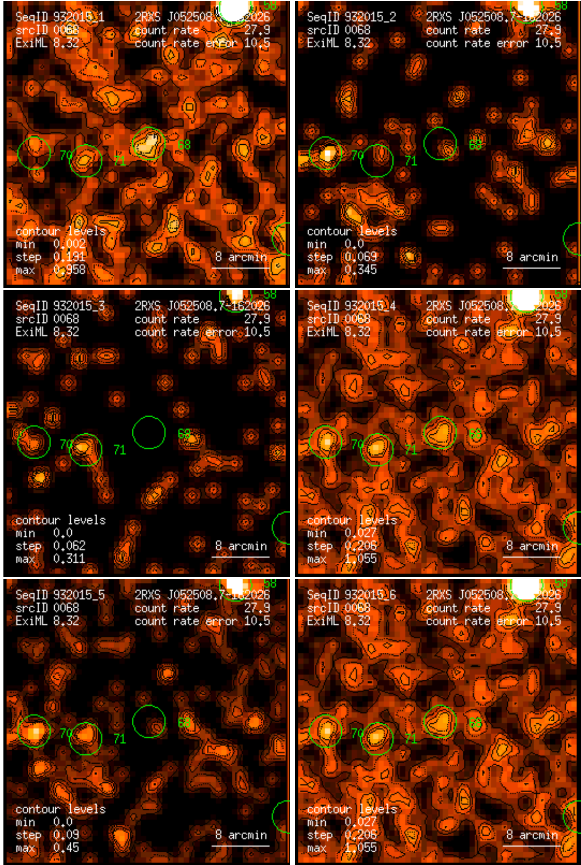
Figure 68: RASS 932015: detection 0068: band rate images, Gaussian filter: (1) PSPC channels 11 – 41, (2) 52 – 90, (3) 91 – 201, (4) 11 – 235, (5) 52 – 201, (6) 11 – 201. Broad band rates in counts/ks. Band rate contour levels in counts/ks/arcmin 2 .
