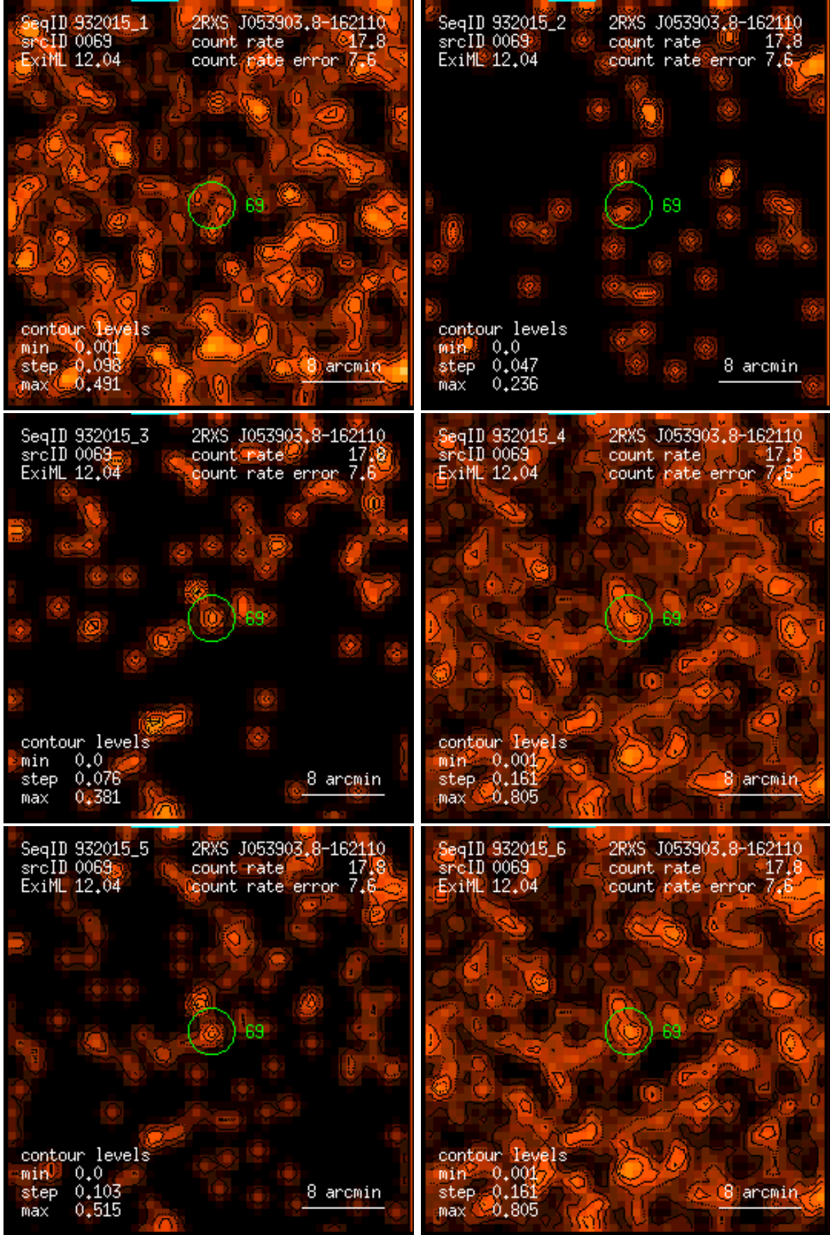
Figure 69: RASS 932015: detection 0069: band rate images, Gaussian filter: (1) PSPC channels 11 – 41, (2) 52 – 90, (3) 91 – 201, (4) 11 – 235, (5) 52 – 201, (6) 11 – 201. Broad band rates in counts/ks. Band rate contour levels in counts/ks/arcmin 2 .
