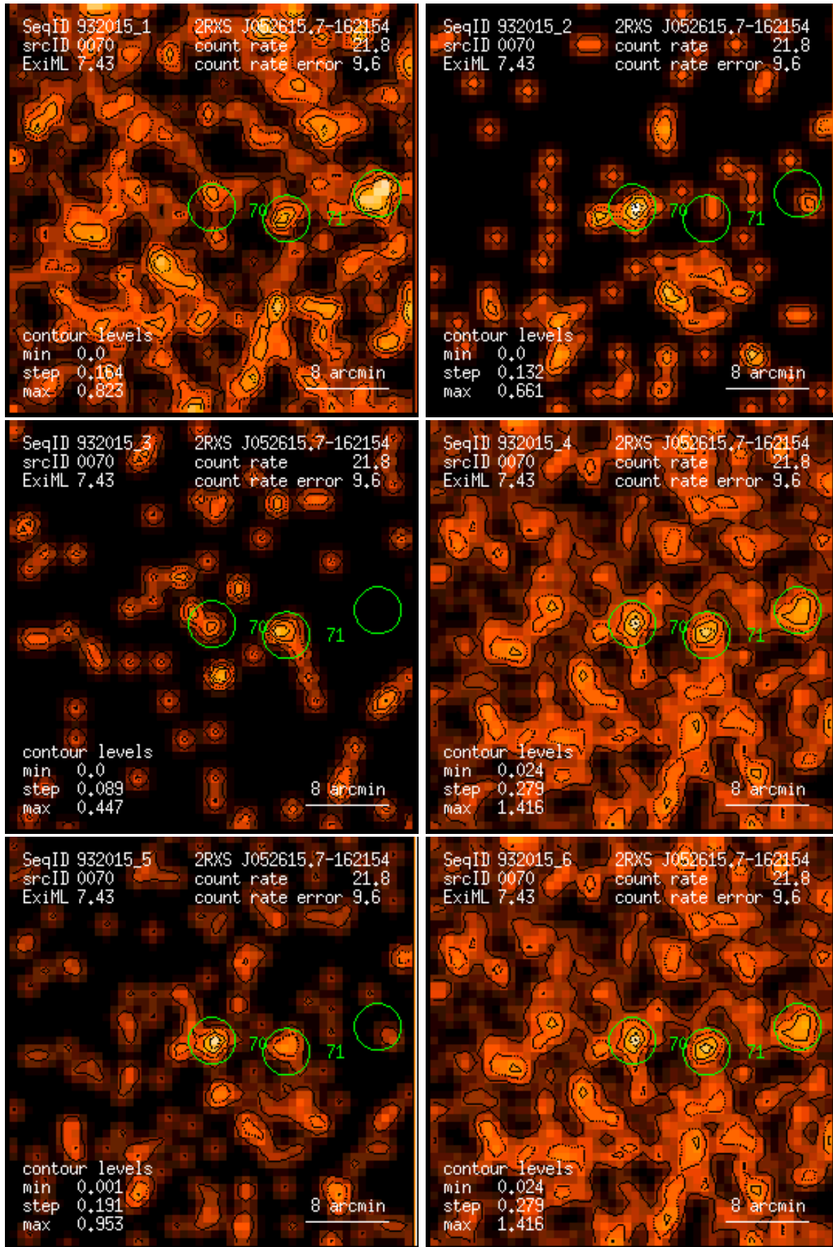
Figure 70: RASS 932015: detection 0070: band rate images, Gaussian filter: (1) PSPC channels 11 – 41, (2) 52 – 90, (3) 91 – 201, (4) 11 – 235, (5) 52 – 201, (6) 11 – 201. Broad band rates in counts/ks. Band rate contour levels in counts/ks/arcmin 2 .
