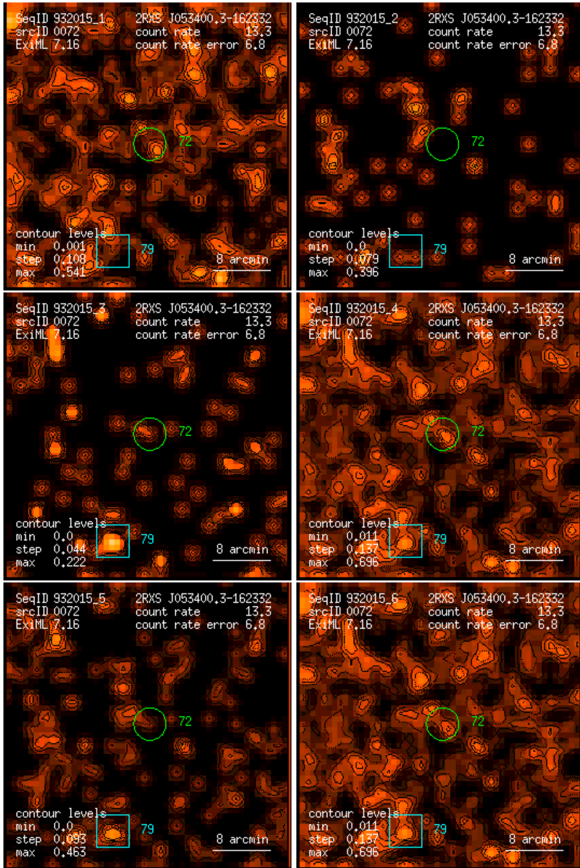
Figure 72: RASS 932015: detection 0072: band rate images, Gaussian filter: (1) PSPC channels 11 – 41, (2) 52 – 90, (3) 91 – 201, (4) 11 – 235, (5) 52 – 201, (6) 11 – 201. Broad band rates in counts/ks. Band rate contour levels in counts/ks/arcmin 2 .
