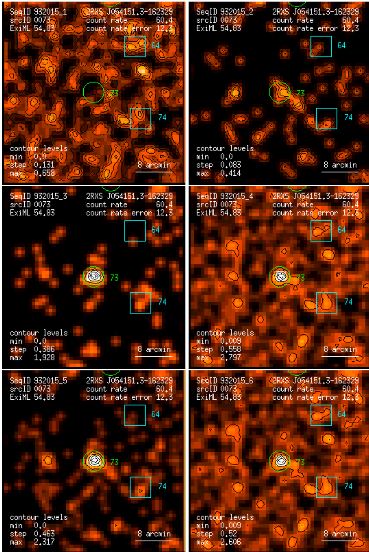
Figure 73: RASS 932015: detection 0073: band rate images, Gaussian filter: (1) PSPC channels 11 – 41, (2) 52 – 90, (3) 91 – 201, (4) 11 – 235, (5) 52 – 201, (6) 11 – 201. Broad band rates in counts/ks. Band rate contour levels in counts/ks/arcmin 2 .
