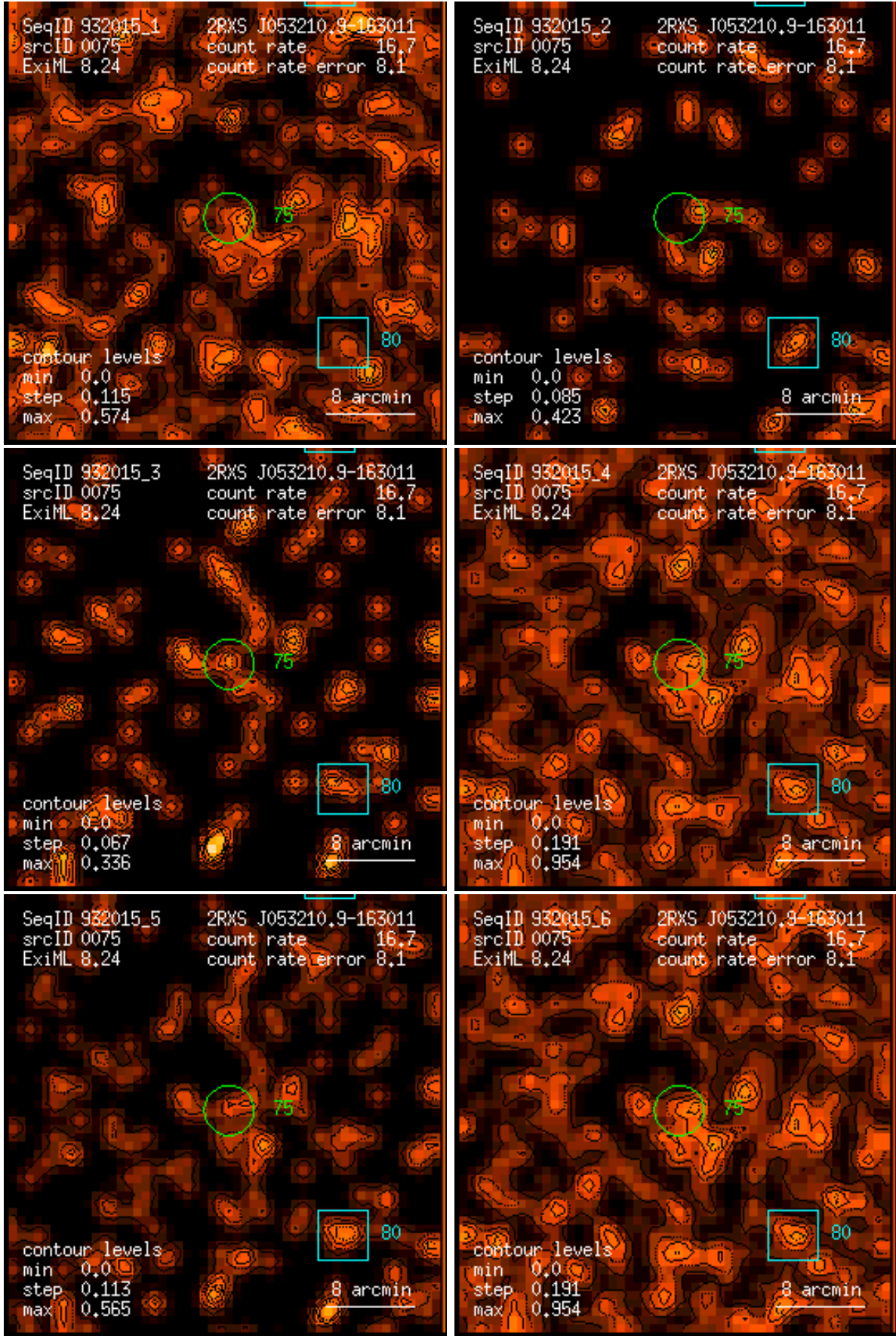
Figure 75: RASS 932015: detection 0075: band rate images, Gaussian filter: (1) PSPC channels 11 – 41, (2) 52 – 90, (3) 91 – 201, (4) 11 – 235, (5) 52 – 201, (6) 11 – 201. Broad band rates in counts/ks. Band rate contour levels in counts/ks/arcmin 2 .
