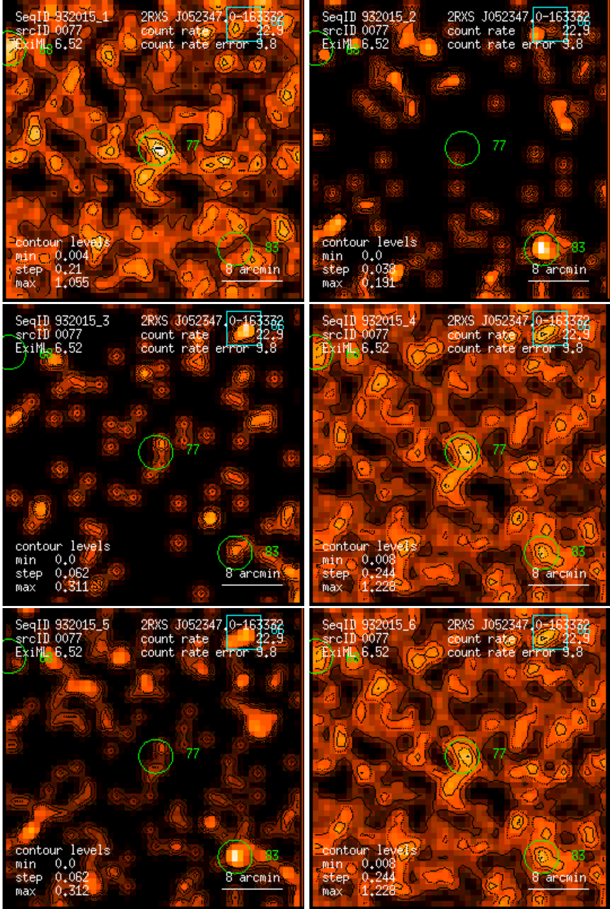
Figure 77: RASS 932015: detection 0077: band rate images, Gaussian filter: (1) PSPC channels 11 – 41, (2) 52 – 90, (3) 91 – 201, (4) 11 – 235, (5) 52 – 201, (6) 11 – 201. Broad band rates in counts/ks. Band rate contour levels in counts/ks/arcmin 2 .
