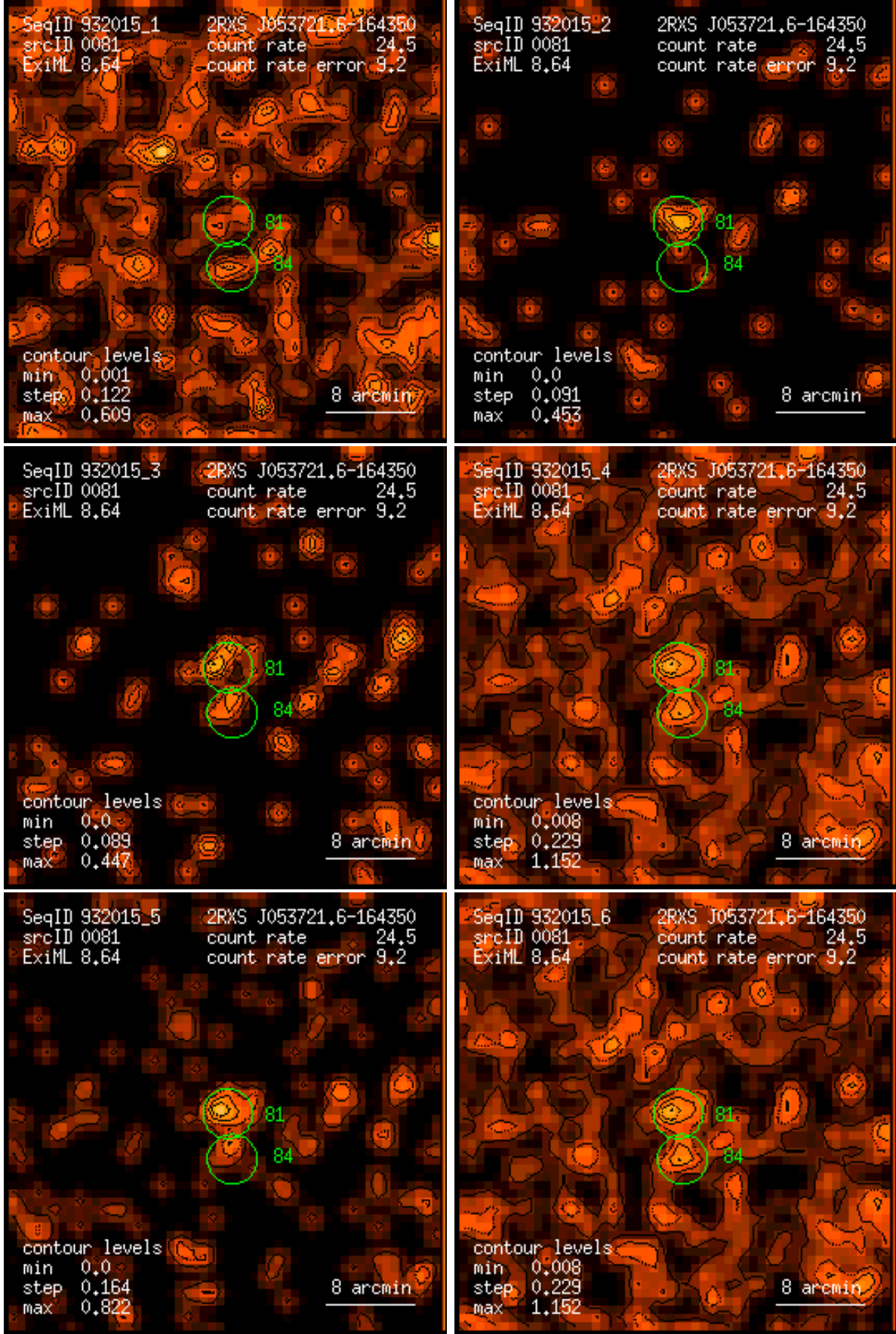
Figure 81: RASS 932015: detection 0081: band rate images, Gaussian filter: (1) PSPC channels 11 – 41, (2) 52 – 90, (3) 91 – 201, (4) 11 – 235, (5) 52 – 201, (6) 11 – 201. Broad band rates in counts/ks. Band rate contour levels in counts/ks/arcmin 2 .
