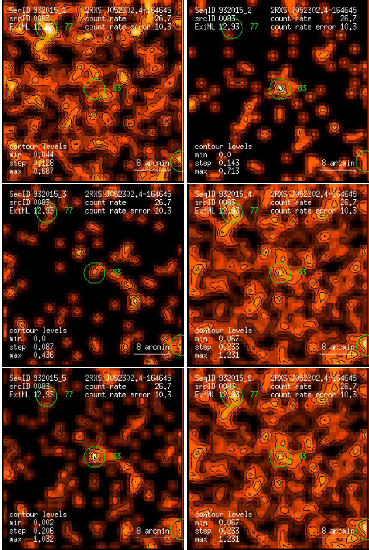
Figure 83: RASS 932015: detection 0083: band rate images, Gaussian filter: (1) PSPC channels 11 – 41, (2) 52 – 90, (3) 91 – 201, (4) 11 – 235, (5) 52 – 201, (6) 11 – 201. Broad band rates in counts/ks. Band rate contour levels in counts/ks/arcmin 2 .
