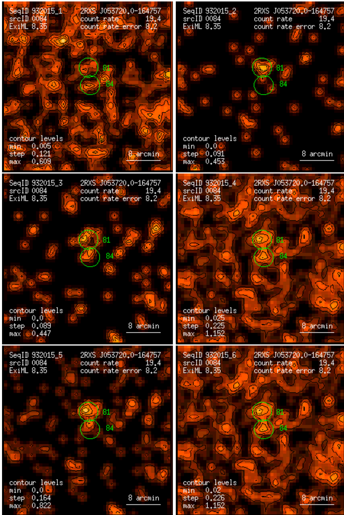
Figure 84: RASS 932015: detection 0084: band rate images, Gaussian filter: (1) PSPC channels 11 – 41, (2) 52 – 90, (3) 91 – 201, (4) 11 – 235, (5) 52 – 201, (6) 11 – 201. Broad band rates in counts/ks. Band rate contour levels in counts/ks/arcmin 2 .
