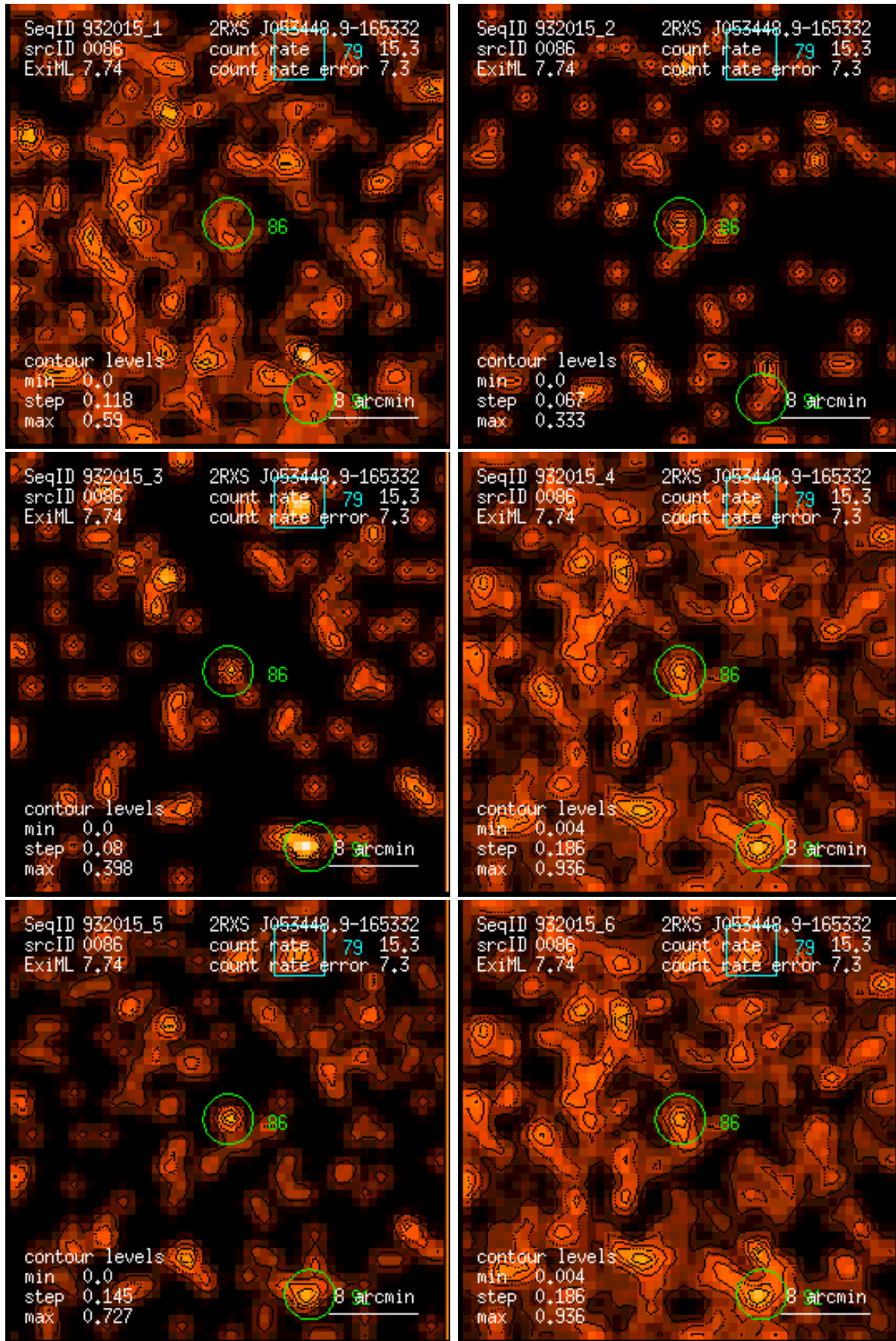
Figure 86: RASS 932015: detection 0086: band rate images, Gaussian filter: (1) PSPC channels 11 – 41, (2) 52 – 90, (3) 91 – 201, (4) 11 – 235, (5) 52 – 201, (6) 11 – 201. Broad band rates in counts/ks. Band rate contour levels in counts/ks/arcmin 2 .
