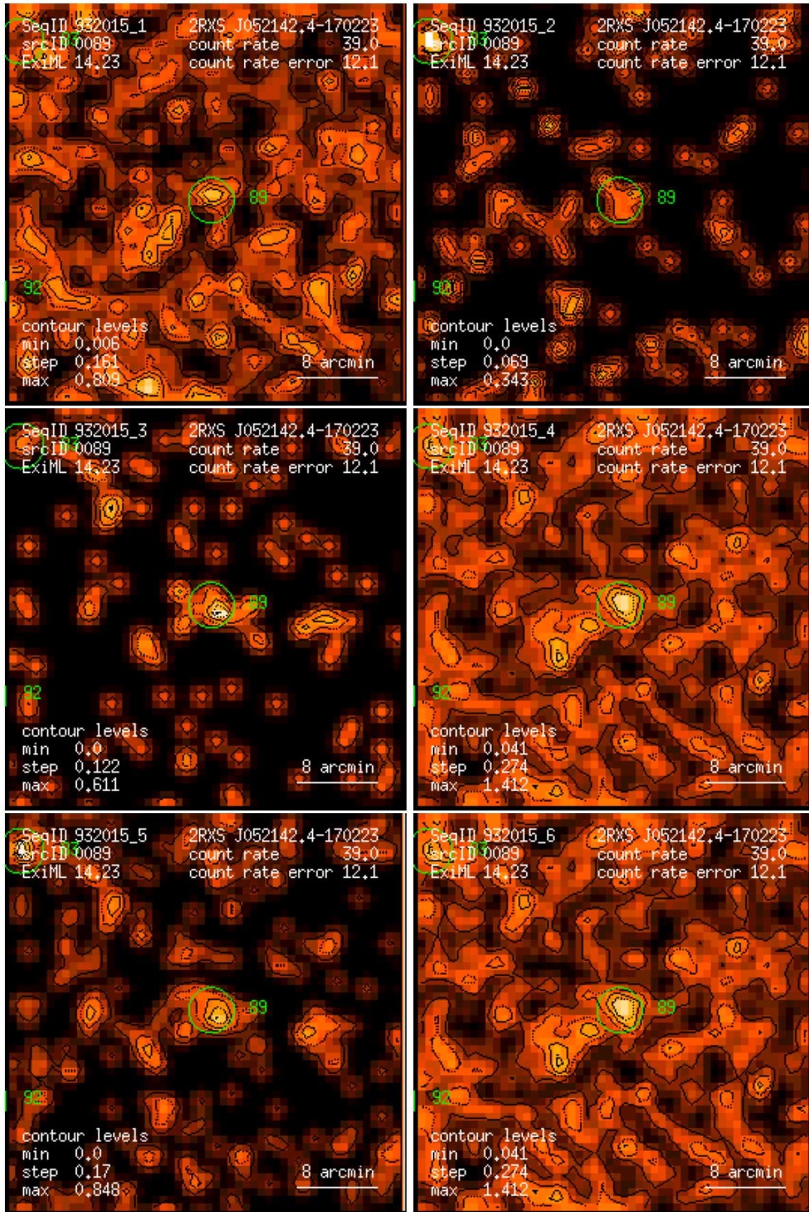
Figure 89: RASS 932015: detection 0089: band rate images, Gaussian filter: (1) PSPC channels 11 – 41, (2) 52 – 90, (3) 91 – 201, (4) 11 – 235, (5) 52 – 201, (6) 11 – 201. Broad band rates in counts/ks. Band rate contour levels in counts/ks/arcmin 2 .
