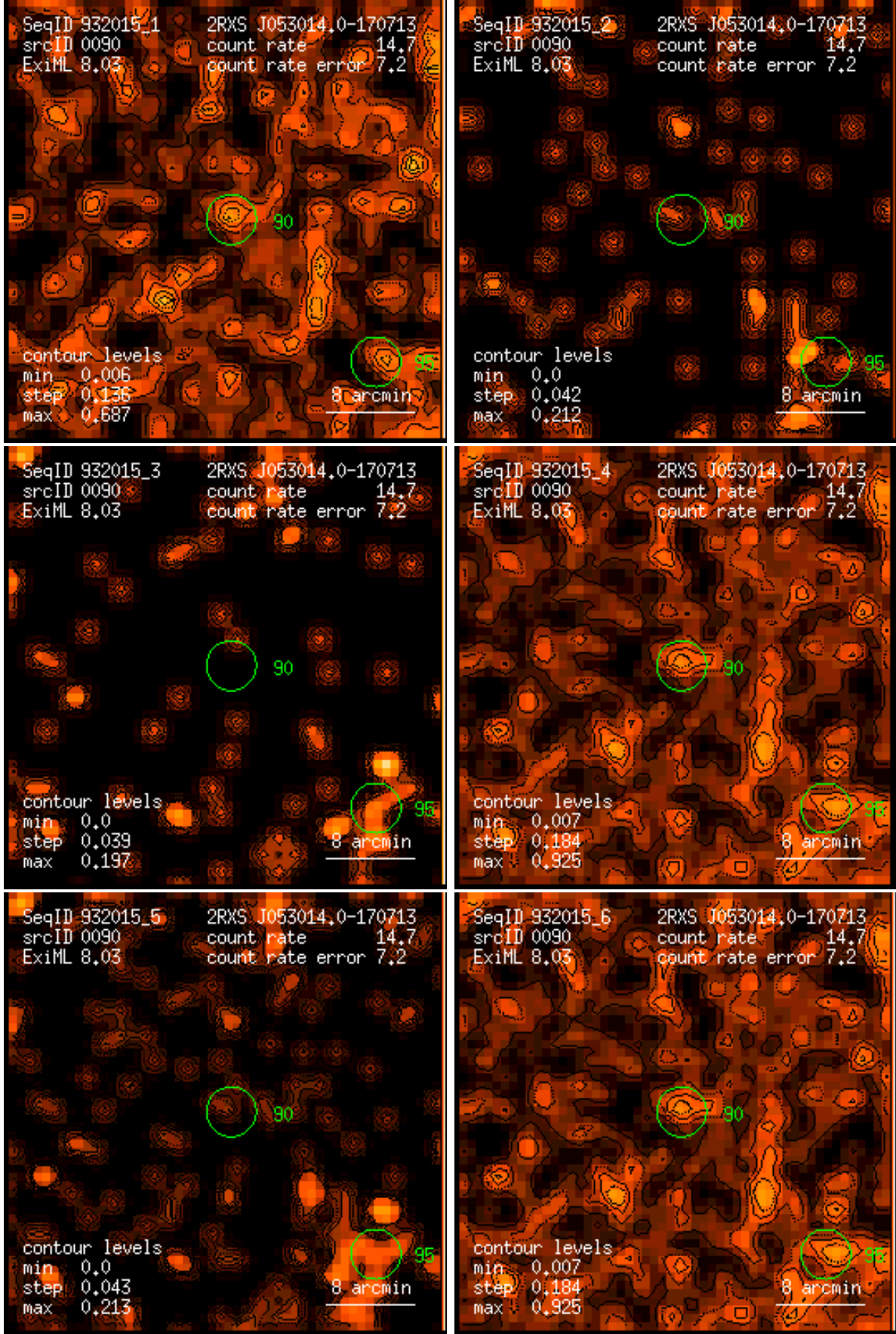
Figure 90: RASS 932015: detection 0090: band rate images, Gaussian filter: (1) PSPC channels 11 – 41, (2) 52 – 90, (3) 91 – 201, (4) 11 – 235, (5) 52 – 201, (6) 11 – 201. Broad band rates in counts/ks. Band rate contour levels in counts/ks/arcmin 2 .
