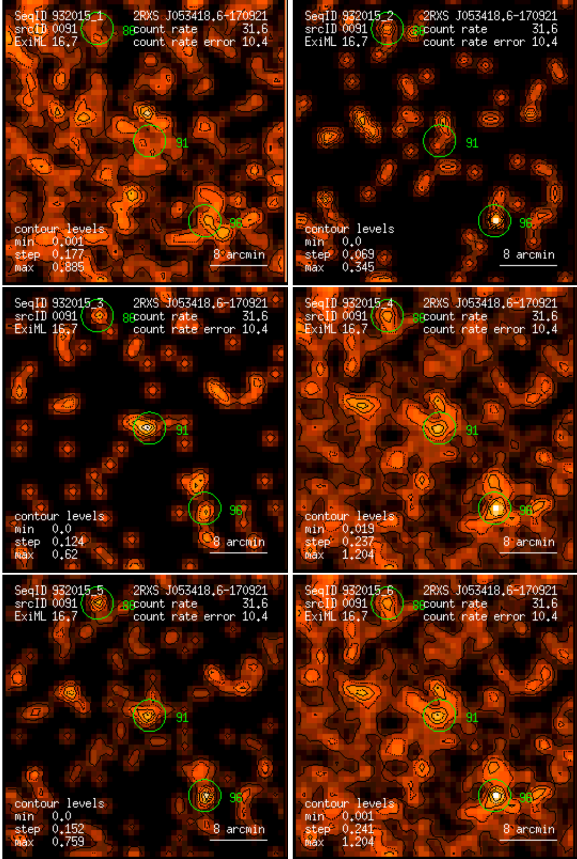
Figure 91: RASS 932015: detection 0091: band rate images, Gaussian filter: (1) PSPC channels 11 – 41, (2) 52 – 90, (3) 91 – 201, (4) 11 – 235, (5) 52 – 201, (6) 11 – 201. Broad band rates in counts/ks. Band rate contour levels in counts/ks/arcmin 2 .
