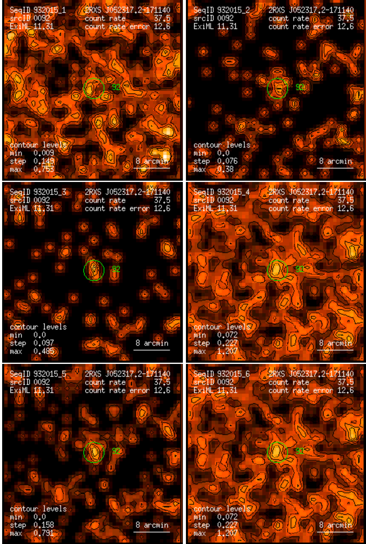
Figure 92: RASS 932015: detection 0092: band rate images, Gaussian filter: (1) PSPC channels 11 – 41, (2) 52 – 90, (3) 91 – 201, (4) 11 – 235, (5) 52 – 201, (6) 11 – 201. Broad band rates in counts/ks. Band rate contour levels in counts/ks/arcmin 2 .
