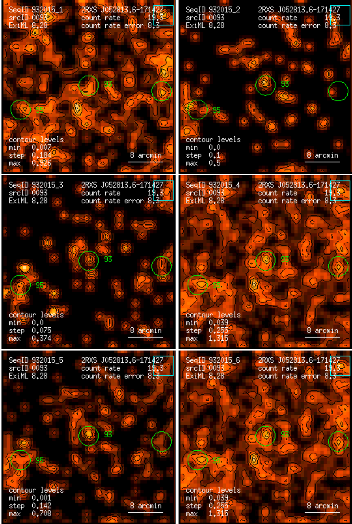
Figure 93: RASS 932015: detection 0093: band rate images, Gaussian filter: (1) PSPC channels 11 – 41, (2) 52 – 90, (3) 91 – 201, (4) 11 – 235, (5) 52 – 201, (6) 11 – 201. Broad band rates in counts/ks. Band rate contour levels in counts/ks/arcmin 2 .
