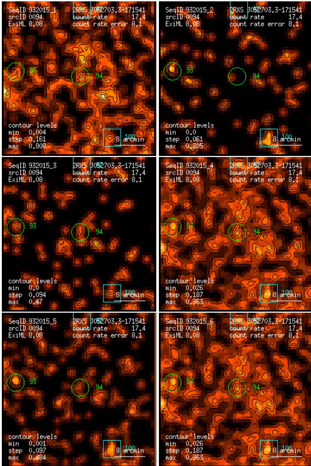
Figure 94: RASS 932015: detection 0094: band rate images, Gaussian filter: (1) PSPC channels 11 – 41, (2) 52 – 90, (3) 91 – 201, (4) 11 – 235, (5) 52 – 201, (6) 11 – 201. Broad band rates in counts/ks. Band rate contour levels in counts/ks/arcmin 2 .
