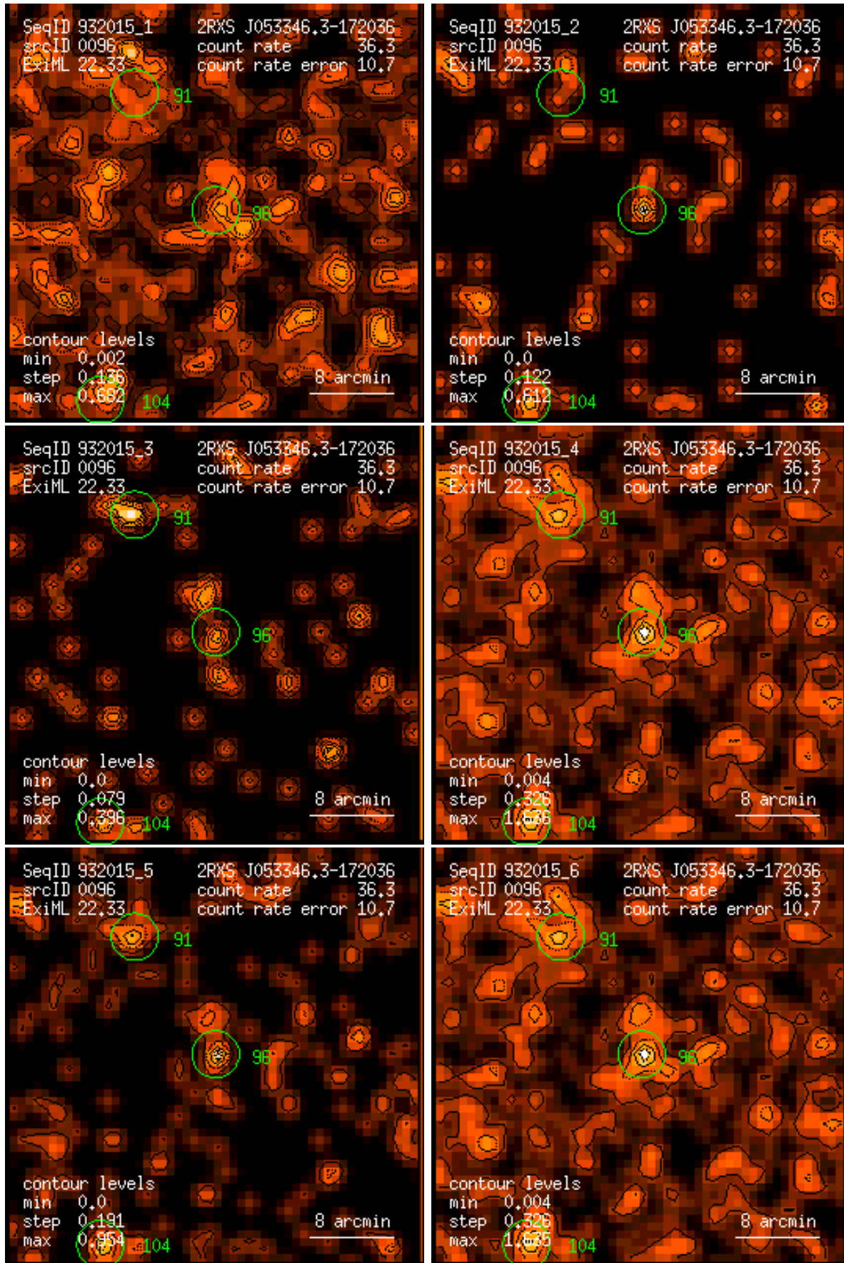
Figure 96: RASS 932015: detection 0096: band rate images, Gaussian filter: (1) PSPC channels 11 – 41, (2) 52 – 90, (3) 91 – 201, (4) 11 – 235, (5) 52 – 201, (6) 11 – 201. Broad band rates in counts/ks. Band rate contour levels in counts/ks/arcmin 2 .
