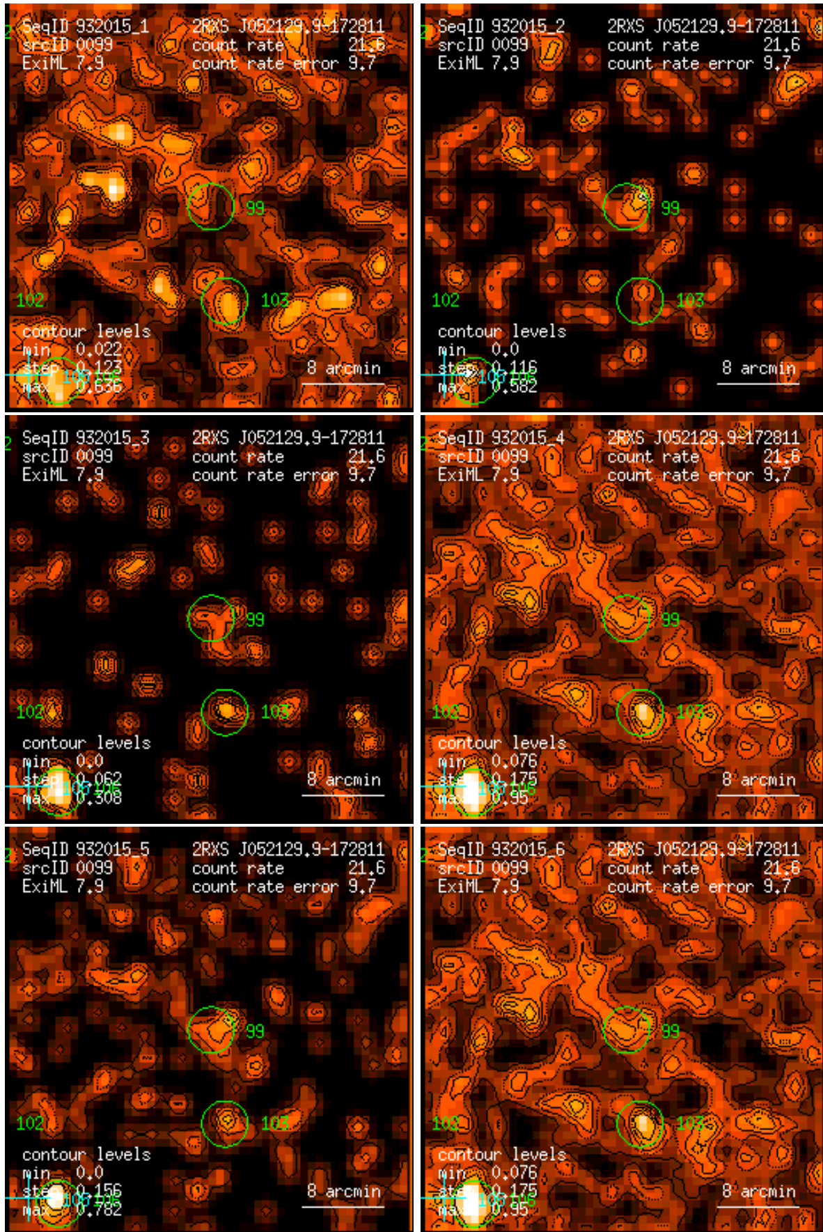
Figure 99: RASS 932015: detection 0099: band rate images, Gaussian filter: (1) PSPC channels 11 – 41, (2) 52 – 90, (3) 91 – 201, (4) 11 – 235, (5) 52 – 201, (6) 11 – 201. Broad band rates in counts/ks. Band rate contour levels in counts/ks/arcmin 2 .
