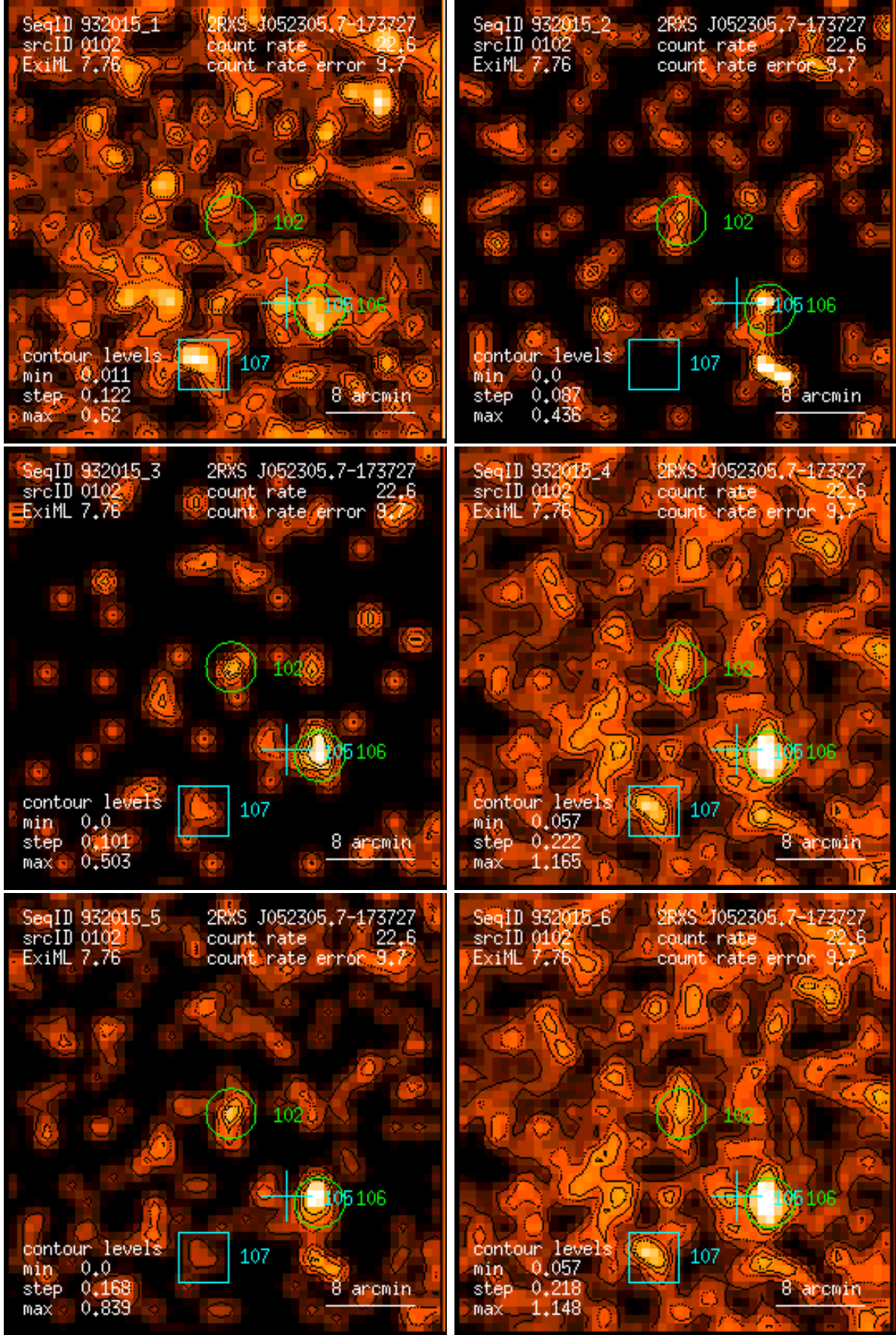
Figure 102: RASS 932015: detection 0102: band rate images, Gaussian filter: (1) PSPC channels 11 – 41, (2) 52 – 90, (3) 91 – 201, (4) 11 – 235, (5) 52 – 201, (6) 11 – 201. Broad band rates in counts/ks. Band rate contour levels in counts/ks/arcmin 2 .
