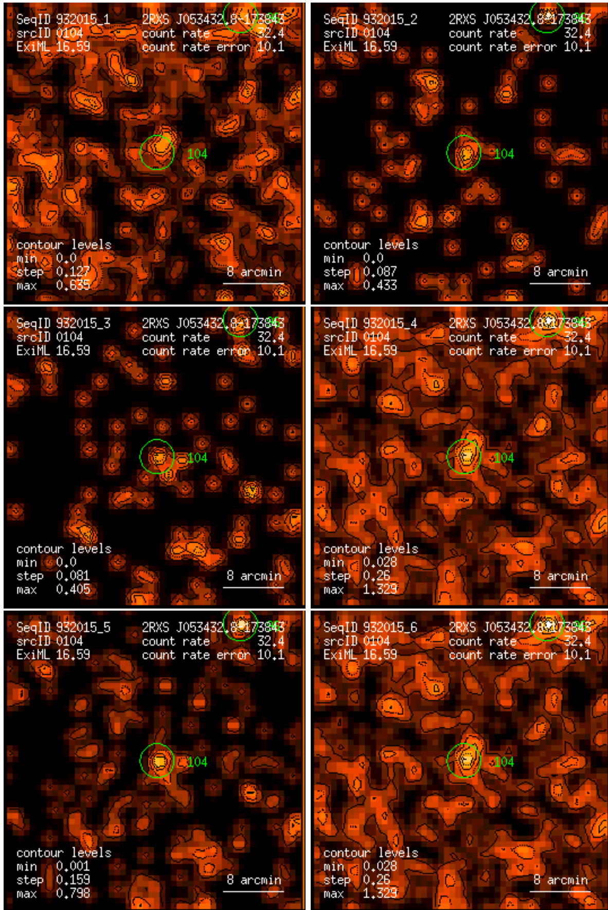
Figure 104: RASS 932015: detection 0104: band rate images, Gaussian filter: (1) PSPC channels 11 – 41, (2) 52 – 90, (3) 91 – 201, (4) 11 – 235, (5) 52 – 201, (6) 11 – 201. Broad band rates in counts/ks. Band rate contour levels in counts/ks/arcmin 2 .
