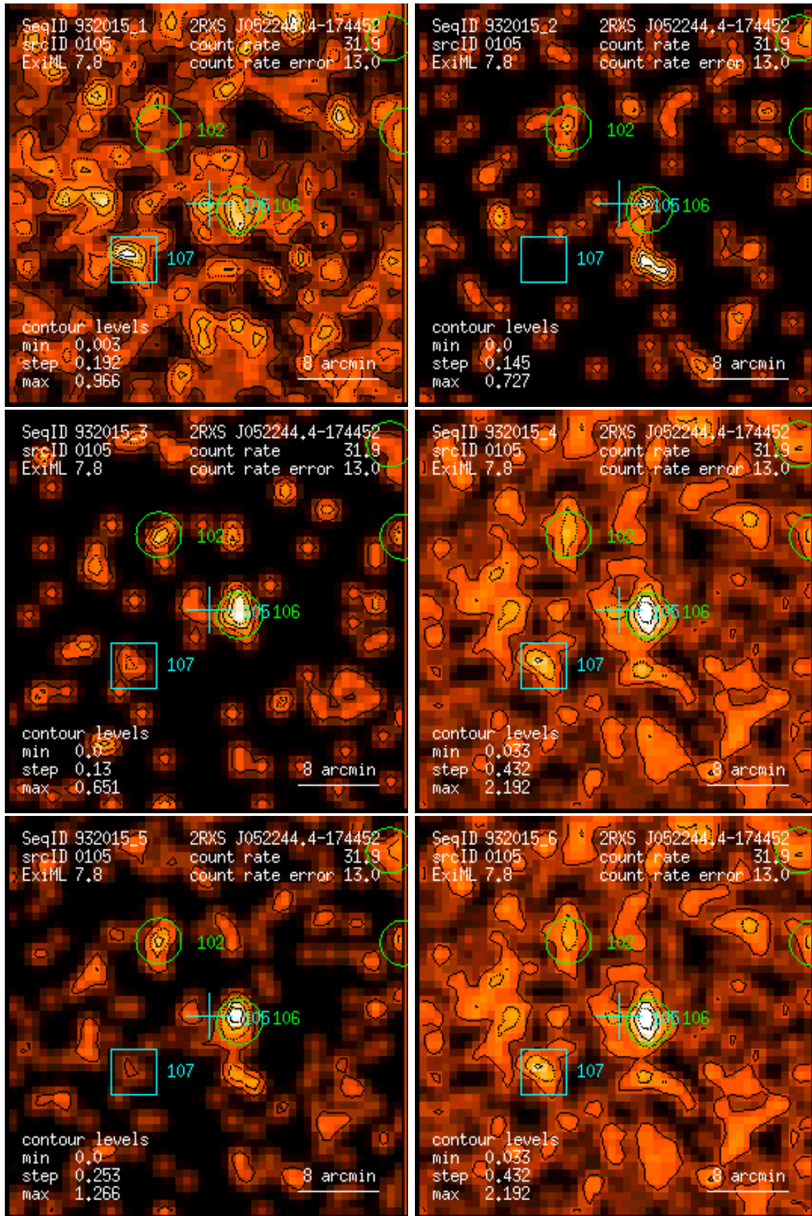
Figure 105: RASS 932015: detection 0105: band rate images, Gaussian filter: (1) PSPC channels 11 – 41, (2) 52 – 90, (3) 91 – 201, (4) 11 – 235, (5) 52 – 201, (6) 11 – 201. Broad band rates in counts/ks. Band rate contour levels in counts/ks/arcmin 2 .
