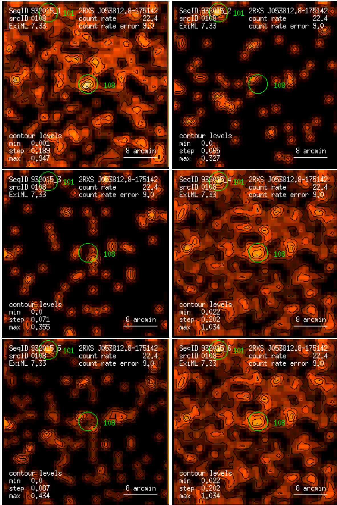
Figure 108: RASS 932015: detection 0108: band rate images, Gaussian filter: (1) PSPC channels 11 – 41, (2) 52 – 90, (3) 91 – 201, (4) 11 – 235, (5) 52 – 201, (6) 11 – 201. Broad band rates in counts/ks. Band rate contour levels in counts/ks/arcmin 2 .
