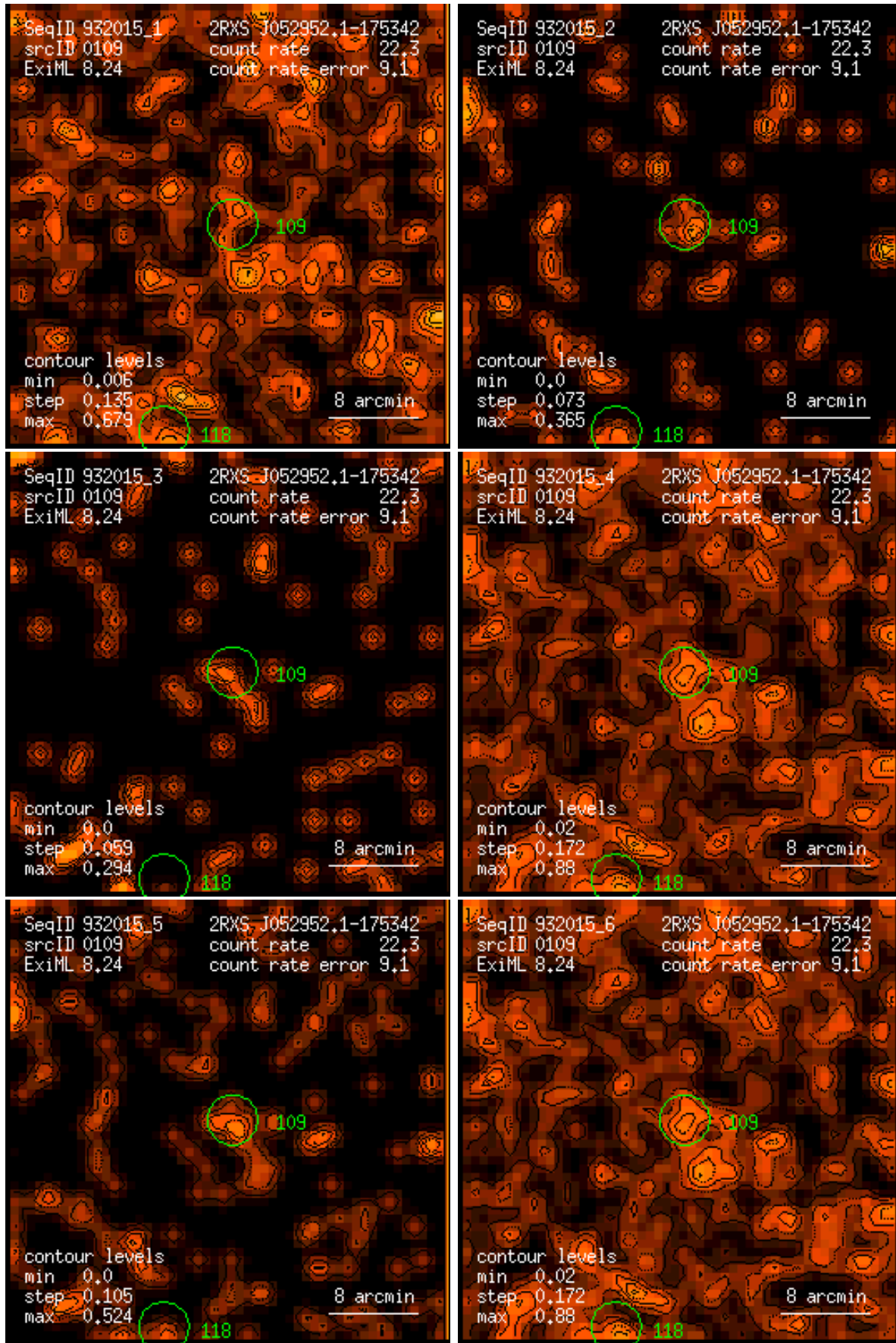
Figure 109: RASS 932015: detection 0109: band rate images, Gaussian filter: (1) PSPC channels 11 – 41, (2) 52 – 90, (3) 91 – 201, (4) 11 – 235, (5) 52 – 201, (6) 11 – 201. Broad band rates in counts/ks. Band rate contour levels in counts/ks/arcmin 2 .
