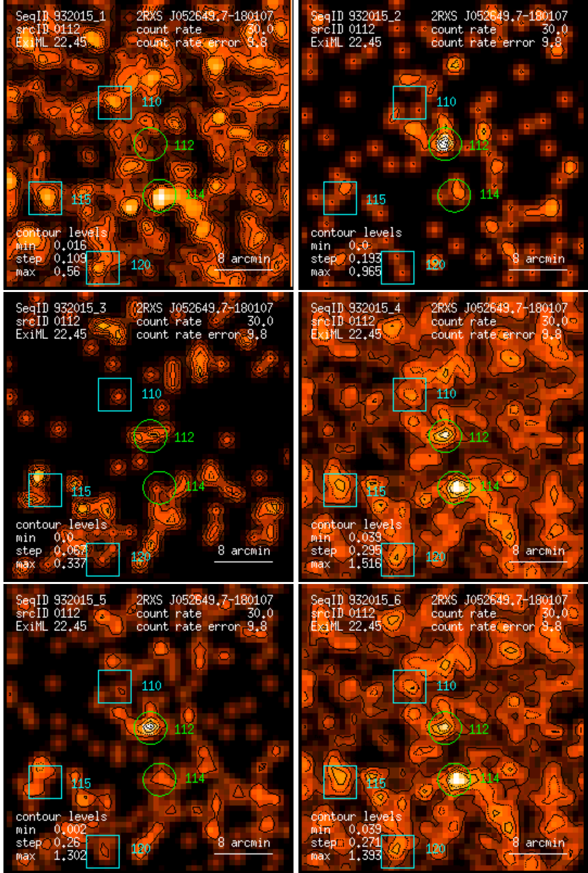
Figure 112: RASS 932015: detection 0112: band rate images, Gaussian filter: (1) PSPC channels 11 – 41, (2) 52 – 90, (3) 91 – 201, (4) 11 – 235, (5) 52 – 201, (6) 11 – 201. Broad band rates in counts/ks. Band rate contour levels in counts/ks/arcmin 2 .
