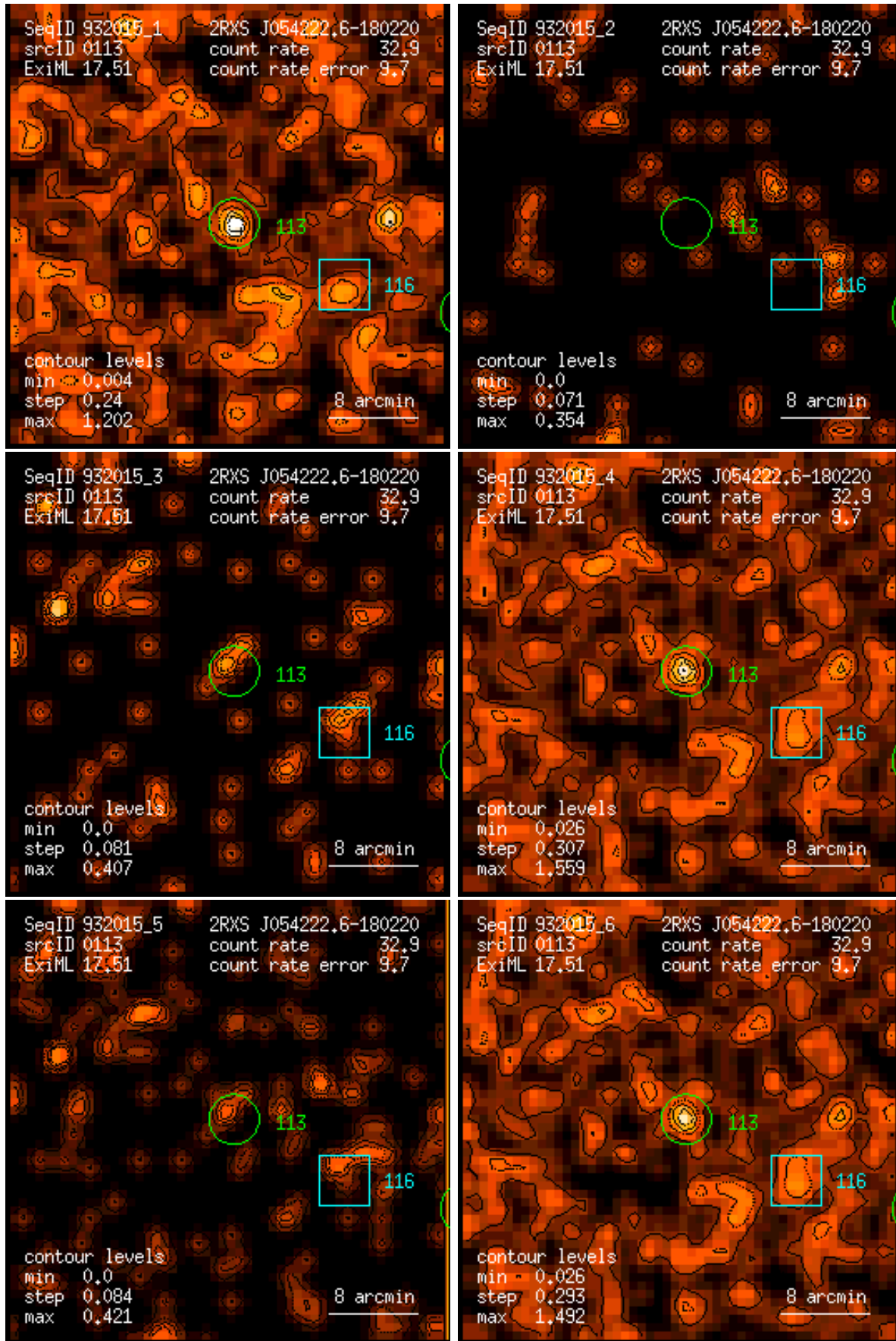
Figure 113: RASS 932015: detection 0113: band rate images, Gaussian filter: (1) PSPC channels 11 – 41, (2) 52 – 90, (3) 91 – 201, (4) 11 – 235, (5) 52 – 201, (6) 11 – 201. Broad band rates in counts/ks. Band rate contour levels in counts/ks/arcmin 2 .
