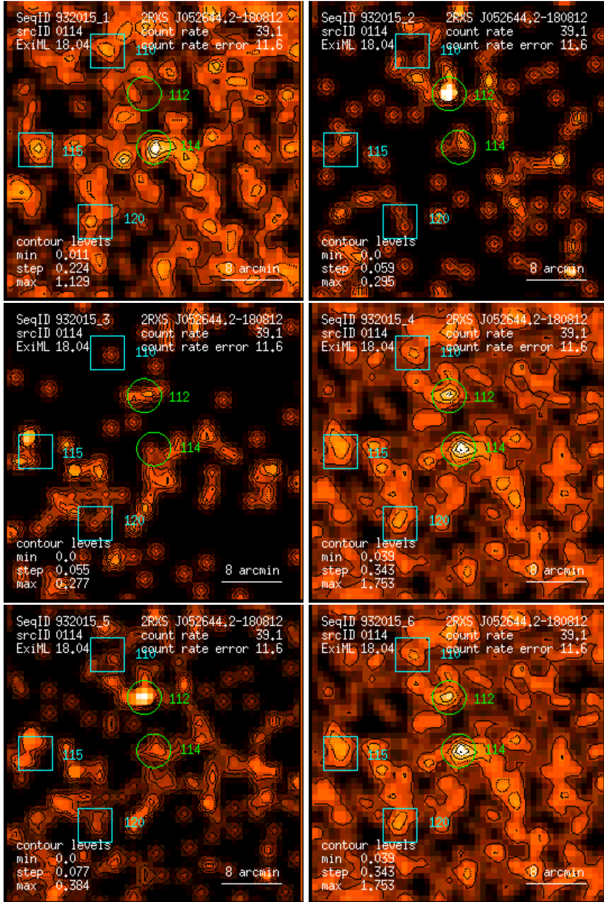
Figure 114: RASS 932015: detection 0114: band rate images, Gaussian filter: (1) PSPC channels 11 – 41, (2) 52 – 90, (3) 91 – 201, (4) 11 – 235, (5) 52 – 201, (6) 11 – 201. Broad band rates in counts/ks. Band rate contour levels in counts/ks/arcmin 2 .
