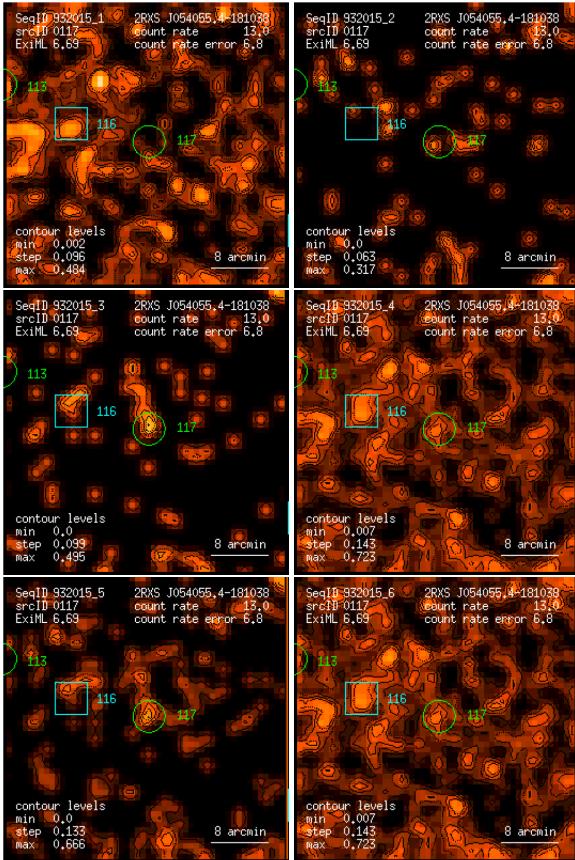
Figure 117: RASS 932015: detection 0117: band rate images, Gaussian filter: (1) PSPC channels 11 – 41, (2) 52 – 90, (3) 91 – 201, (4) 11 – 235, (5) 52 – 201, (6) 11 – 201. Broad band rates in counts/ks. Band rate contour levels in counts/ks/arcmin 2 .
