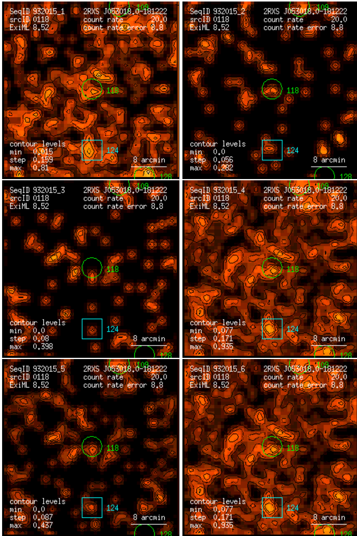
Figure 118: RASS 932015: detection 0118: band rate images, Gaussian filter: (1) PSPC channels 11 – 41, (2) 52 – 90, (3) 91 – 201, (4) 11 – 235, (5) 52 – 201, (6) 11 – 201. Broad band rates in counts/ks. Band rate contour levels in counts/ks/arcmin 2 .
