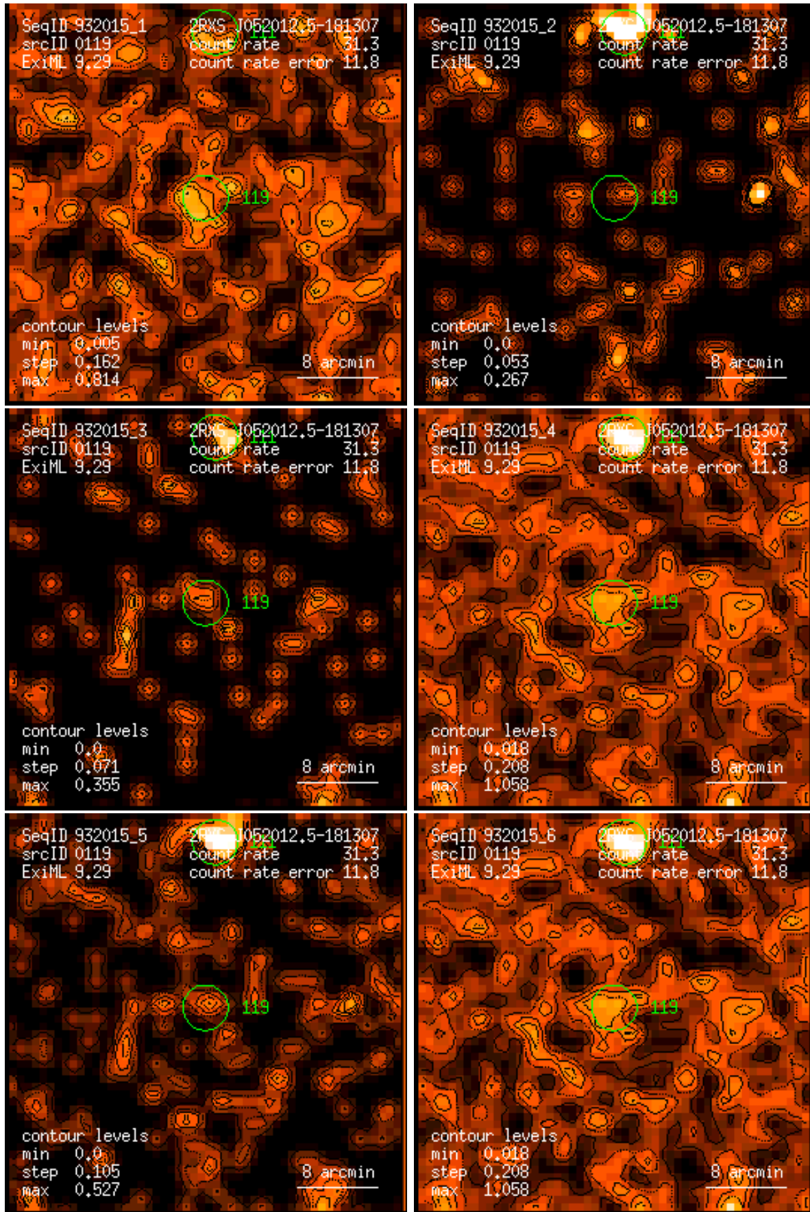
Figure 119: RASS 932015: detection 0119: band rate images, Gaussian filter: (1) PSPC channels 11 – 41, (2) 52 – 90, (3) 91 – 201, (4) 11 – 235, (5) 52 – 201, (6) 11 – 201. Broad band rates in counts/ks. Band rate contour levels in counts/ks/arcmin 2 .
