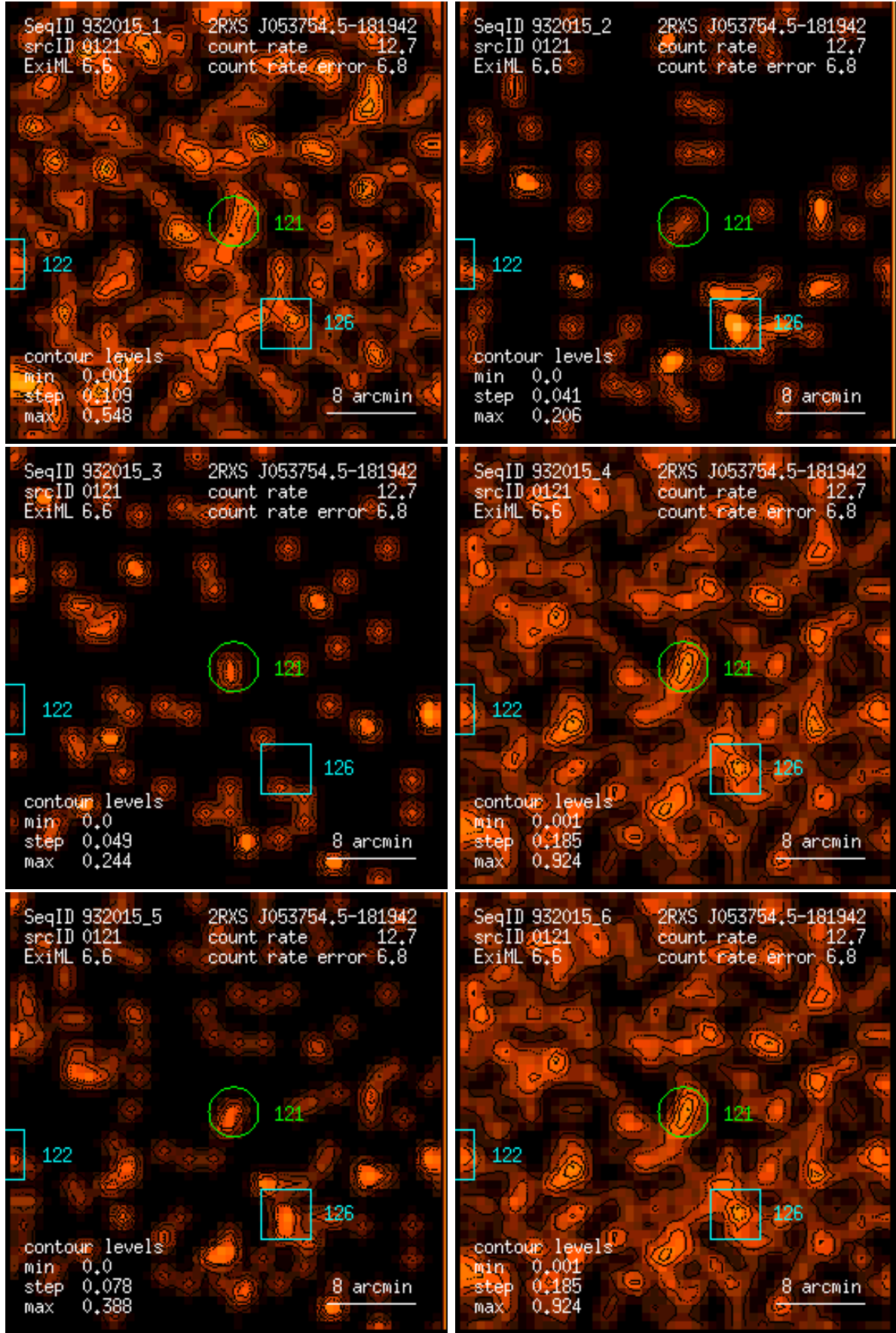
Figure 121: RASS 932015: detection 0121: band rate images, Gaussian filter: (1) PSPC channels 11 – 41, (2) 52 – 90, (3) 91 – 201, (4) 11 – 235, (5) 52 – 201, (6) 11 – 201. Broad band rates in counts/ks. Band rate contour levels in counts/ks/arcmin 2 .
