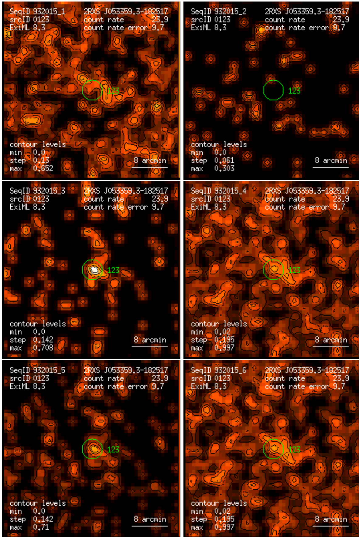
Figure 123: RASS 932015: detection 0123: band rate images, Gaussian filter: (1) PSPC channels 11 – 41, (2) 52 – 90, (3) 91 – 201, (4) 11 – 235, (5) 52 – 201, (6) 11 – 201. Broad band rates in counts/ks. Band rate contour levels in counts/ks/arcmin 2 .
