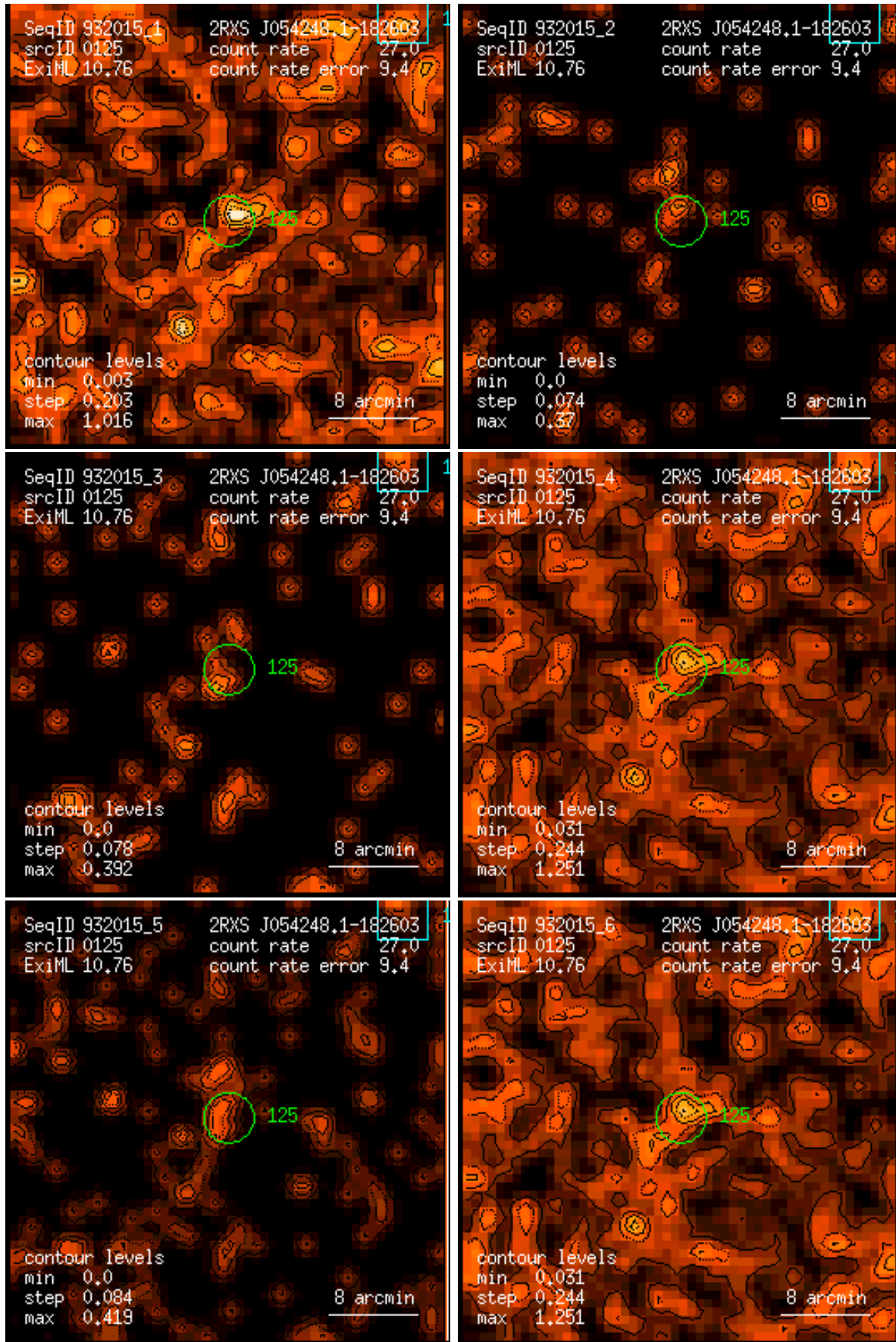
Figure 125: RASS 932015: detection 0125: band rate images, Gaussian filter: (1) PSPC channels 11 – 41, (2) 52 – 90, (3) 91 – 201, (4) 11 – 235, (5) 52 – 201, (6) 11 – 201. Broad band rates in counts/ks. Band rate contour levels in counts/ks/arcmin 2 .
