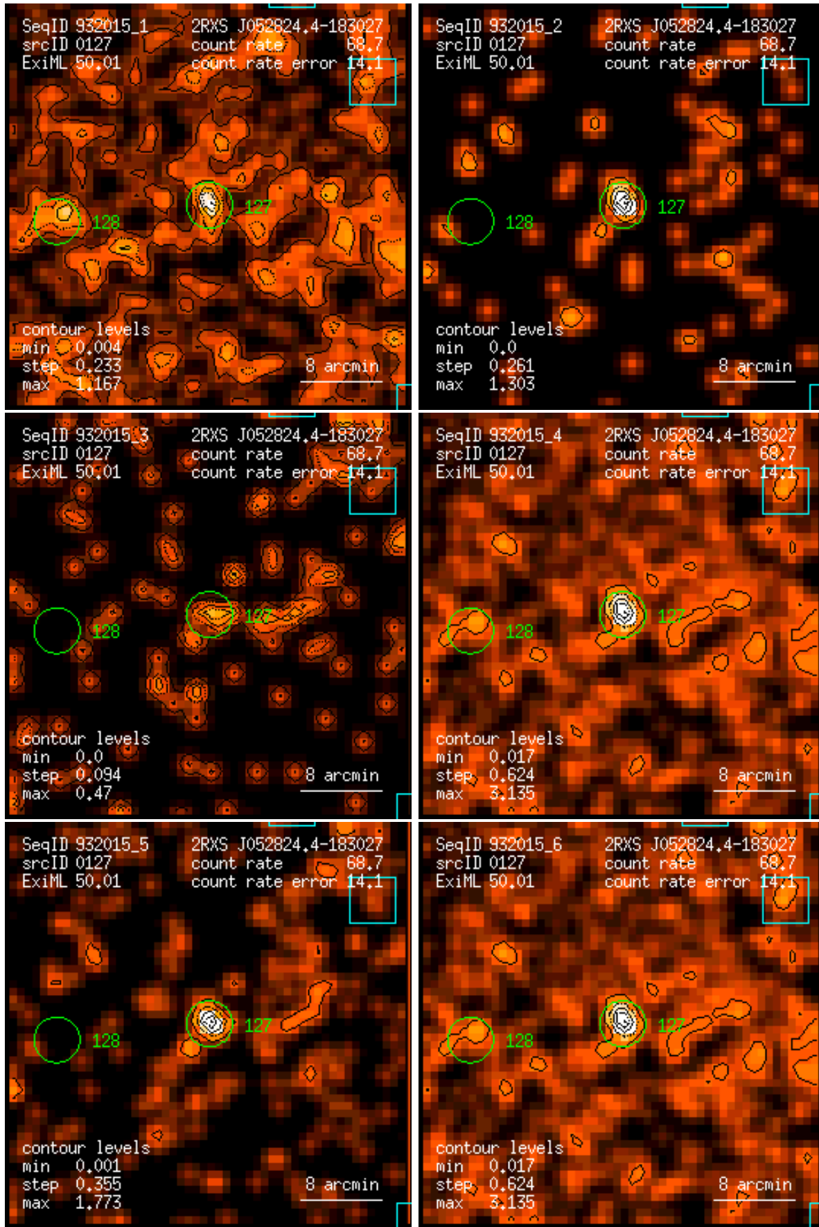
Figure 127: RASS 932015: detection 0127: band rate images, Gaussian filter: (1) PSPC channels 11 – 41, (2) 52 – 90, (3) 91 – 201, (4) 11 – 235, (5) 52 – 201, (6) 11 – 201. Broad band rates in counts/ks. Band rate contour levels in counts/ks/arcmin 2 .
