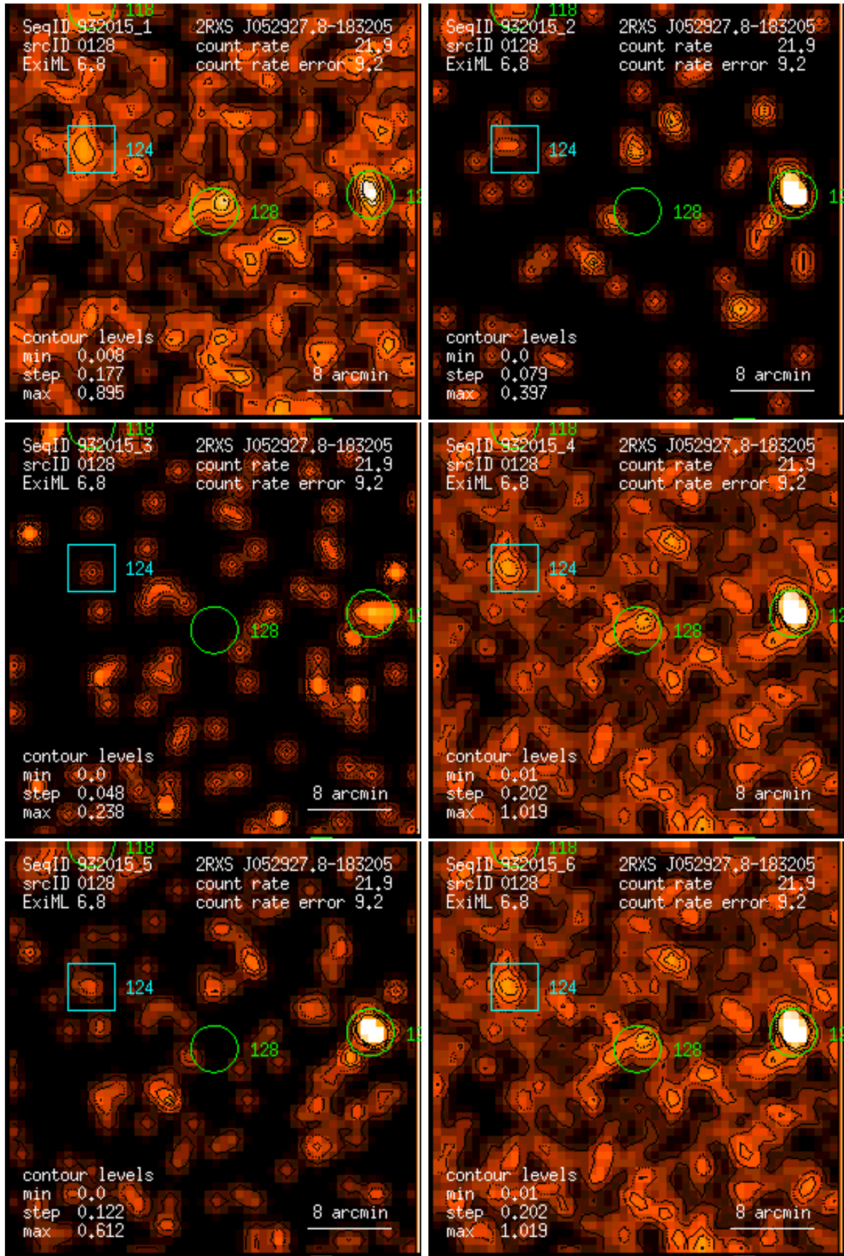
Figure 128: RASS 932015: detection 0128: band rate images, Gaussian filter: (1) PSPC channels 11 – 41, (2) 52 – 90, (3) 91 – 201, (4) 11 – 235, (5) 52 – 201, (6) 11 – 201. Broad band rates in counts/ks. Band rate contour levels in counts/ks/arcmin 2 .
