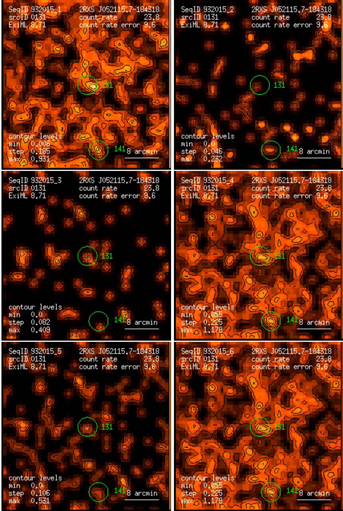
Figure 131: RASS 932015: detection 0131: band rate images, Gaussian filter: (1) PSPC channels 11 – 41, (2) 52 – 90, (3) 91 – 201, (4) 11 – 235, (5) 52 – 201, (6) 11 – 201. Broad band rates in counts/ks. Band rate contour levels in counts/ks/arcmin 2 .
