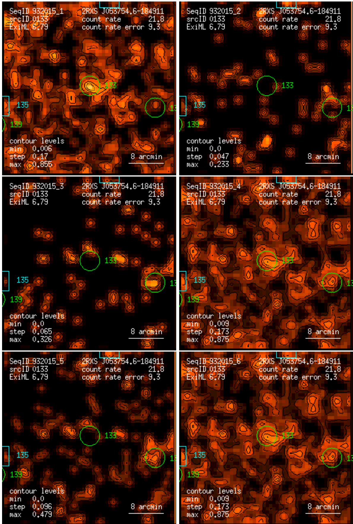
Figure 133: RASS 932015: detection 0133: band rate images, Gaussian filter: (1) PSPC channels 11 – 41, (2) 52 – 90, (3) 91 – 201, (4) 11 – 235, (5) 52 – 201, (6) 11 – 201. Broad band rates in counts/ks. Band rate contour levels in counts/ks/arcmin 2 .
