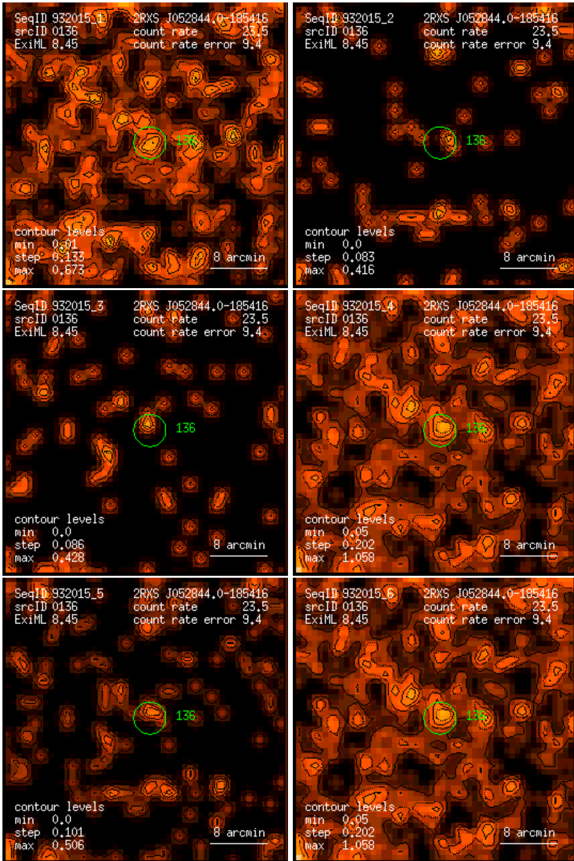
Figure 136: RASS 932015: detection 0136: band rate images, Gaussian filter: (1) PSPC channels 11 – 41, (2) 52 – 90, (3) 91 – 201, (4) 11 – 235, (5) 52 – 201, (6) 11 – 201. Broad band rates in counts/ks. Band rate contour levels in counts/ks/arcmin 2 .
