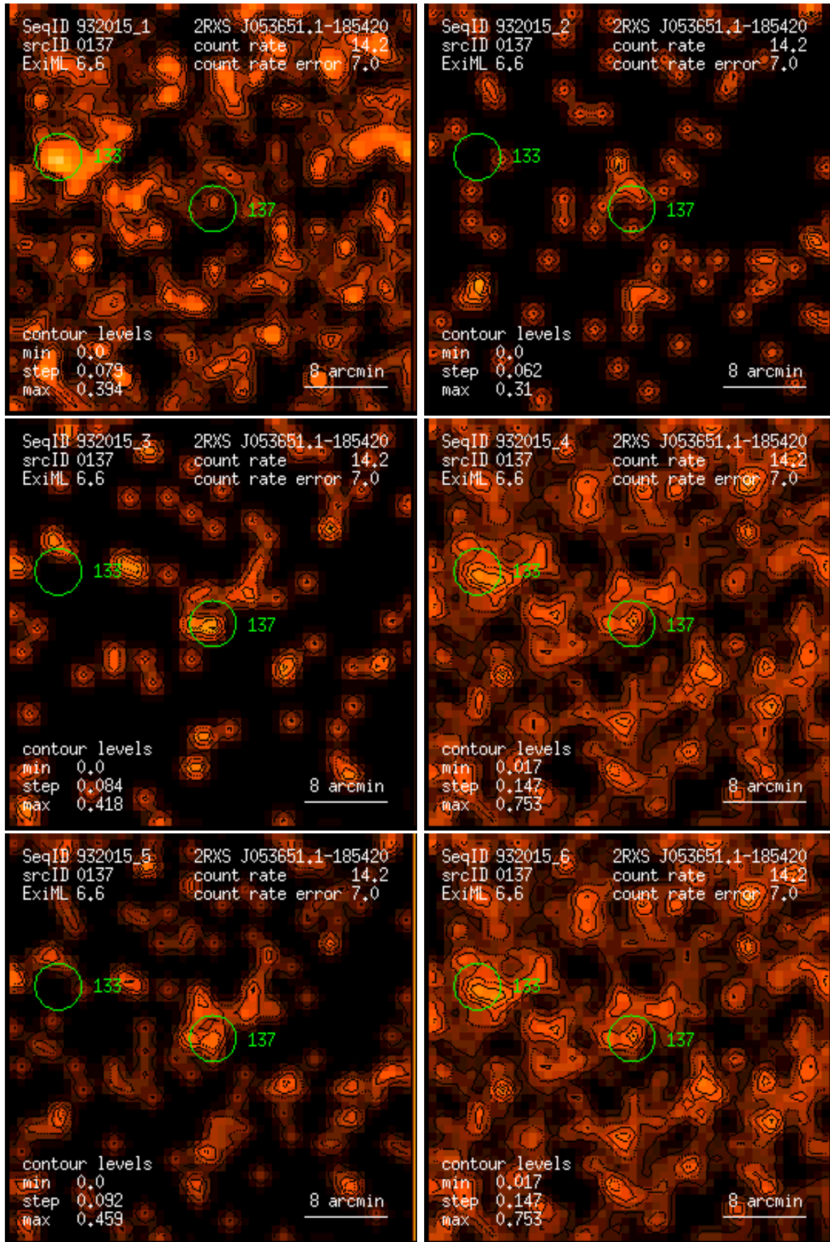
Figure 137: RASS 932015: detection 0137: band rate images, Gaussian filter: (1) PSPC channels 11 – 41, (2) 52 – 90, (3) 91 – 201, (4) 11 – 235, (5) 52 – 201, (6) 11 – 201. Broad band rates in counts/ks. Band rate contour levels in counts/ks/arcmin 2 .
