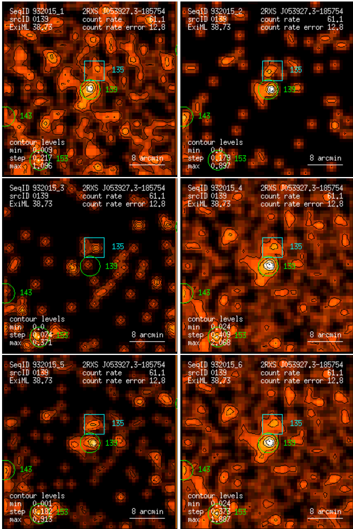
Figure 139: RASS 932015: detection 0139: band rate images, Gaussian filter: (1) PSPC channels 11 – 41, (2) 52 – 90, (3) 91 – 201, (4) 11 – 235, (5) 52 – 201, (6) 11 – 201. Broad band rates in counts/ks. Band rate contour levels in counts/ks/arcmin 2 .
