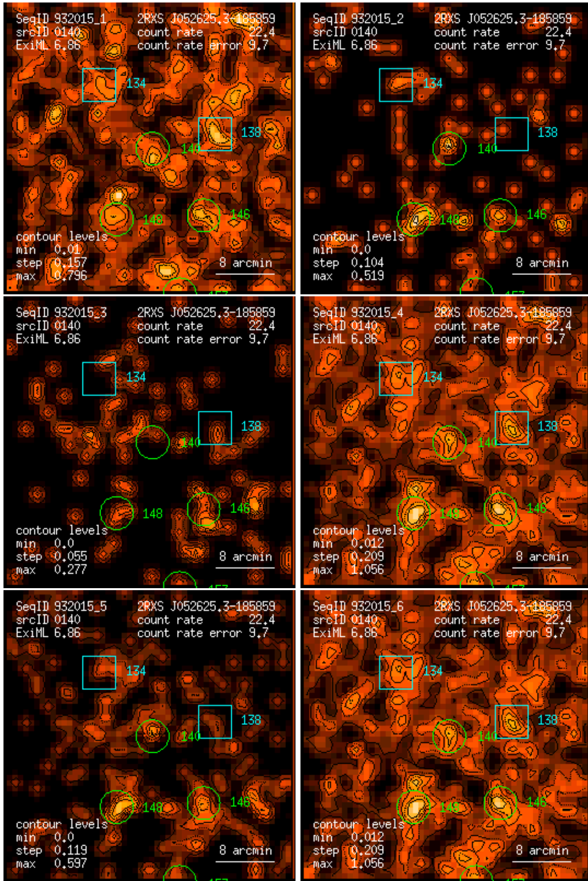
Figure 140: RASS 932015: detection 0140: band rate images, Gaussian filter: (1) PSPC channels 11 – 41, (2) 52 – 90, (3) 91 – 201, (4) 11 – 235, (5) 52 – 201, (6) 11 – 201. Broad band rates in counts/ks. Band rate contour levels in counts/ks/arcmin 2 .
