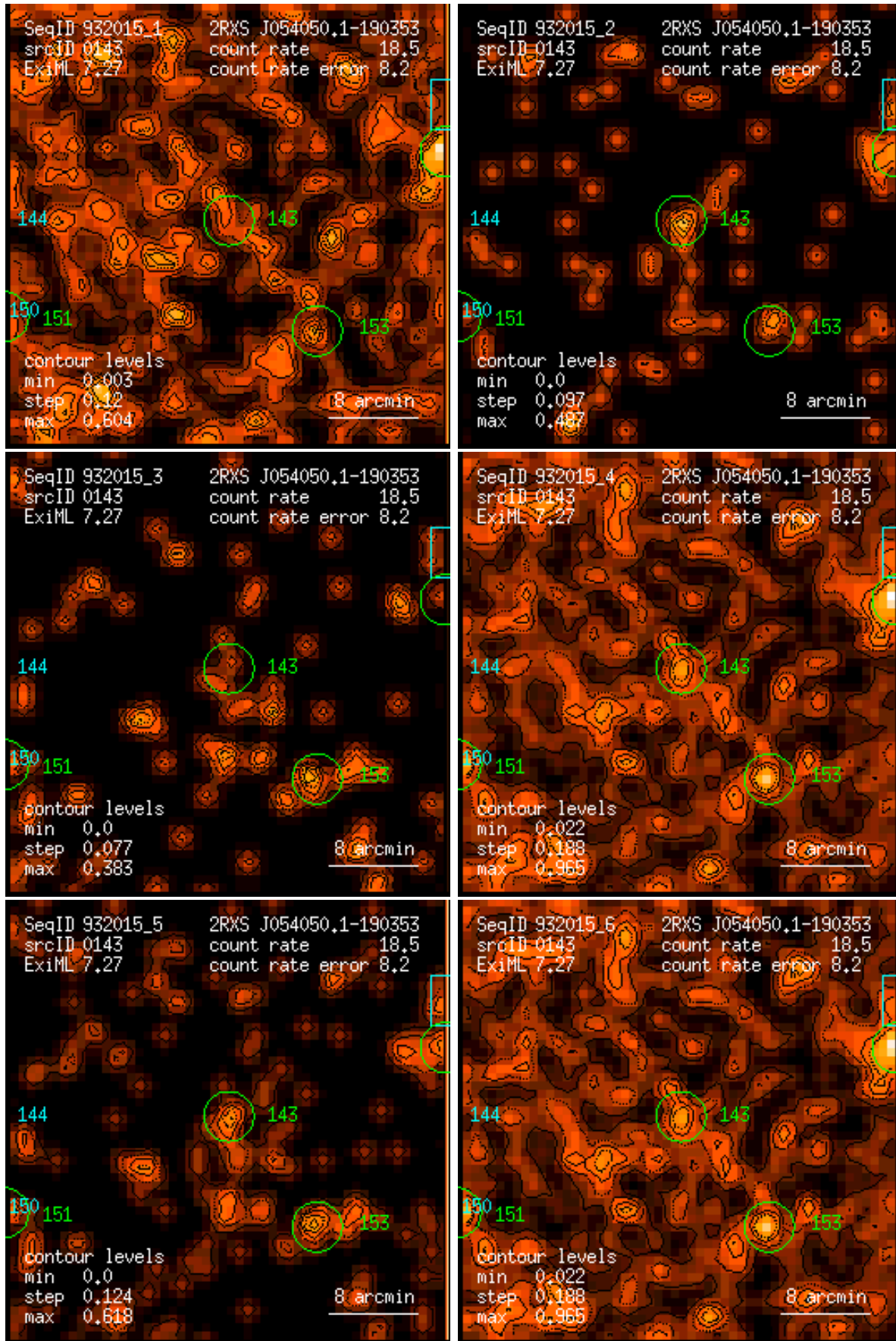
Figure 143: RASS 932015: detection 0143: band rate images, Gaussian filter: (1) PSPC channels 11 – 41, (2) 52 – 90, (3) 91 – 201, (4) 11 – 235, (5) 52 – 201, (6) 11 – 201. Broad band rates in counts/ks. Band rate contour levels in counts/ks/arcmin 2 .
