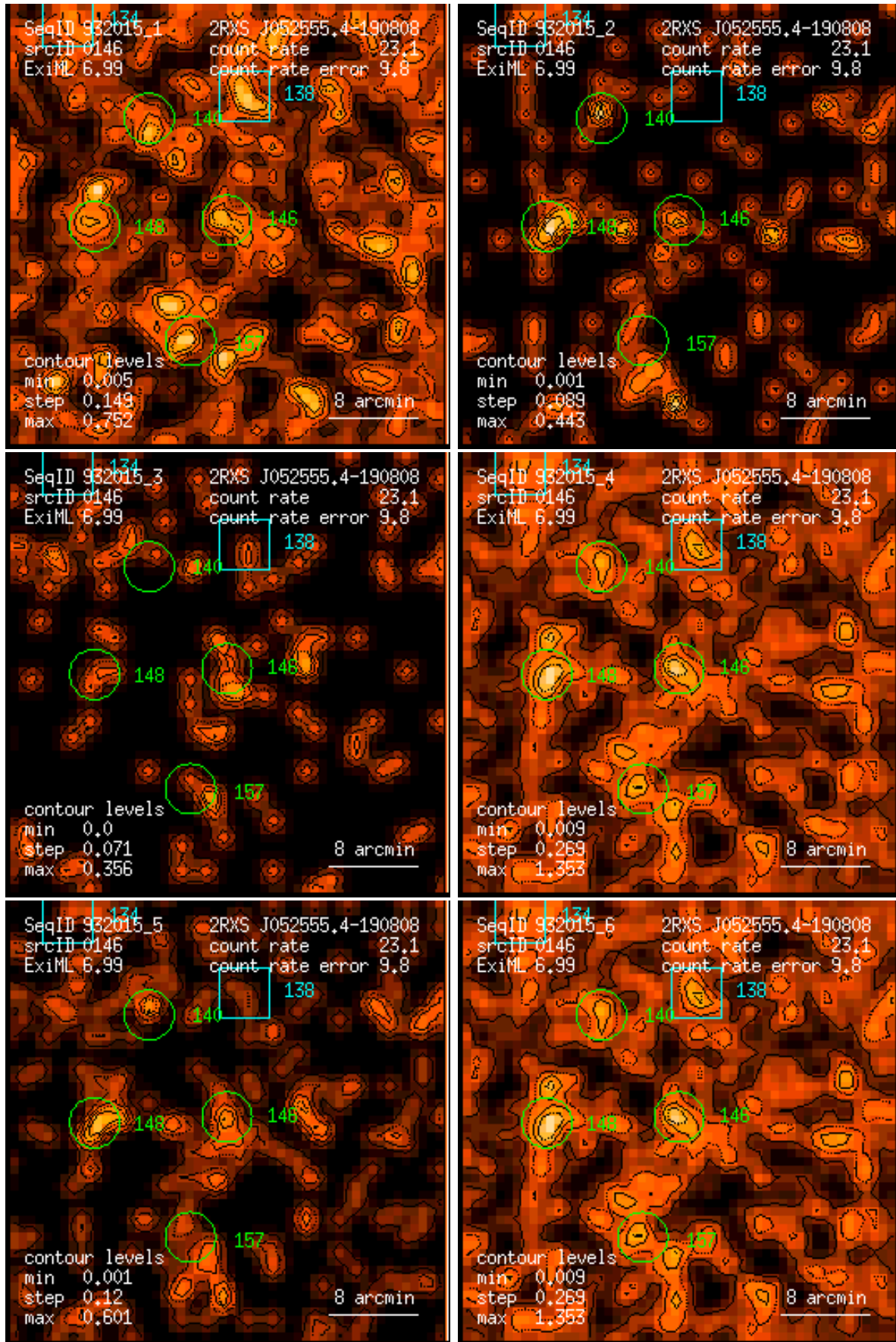
Figure 146: RASS 932015: detection 0146: band rate images, Gaussian filter: (1) PSPC channels 11 – 41, (2) 52 – 90, (3) 91 – 201, (4) 11 – 235, (5) 52 – 201, (6) 11 – 201. Broad band rates in counts/ks. Band rate contour levels in counts/ks/arcmin 2 .
