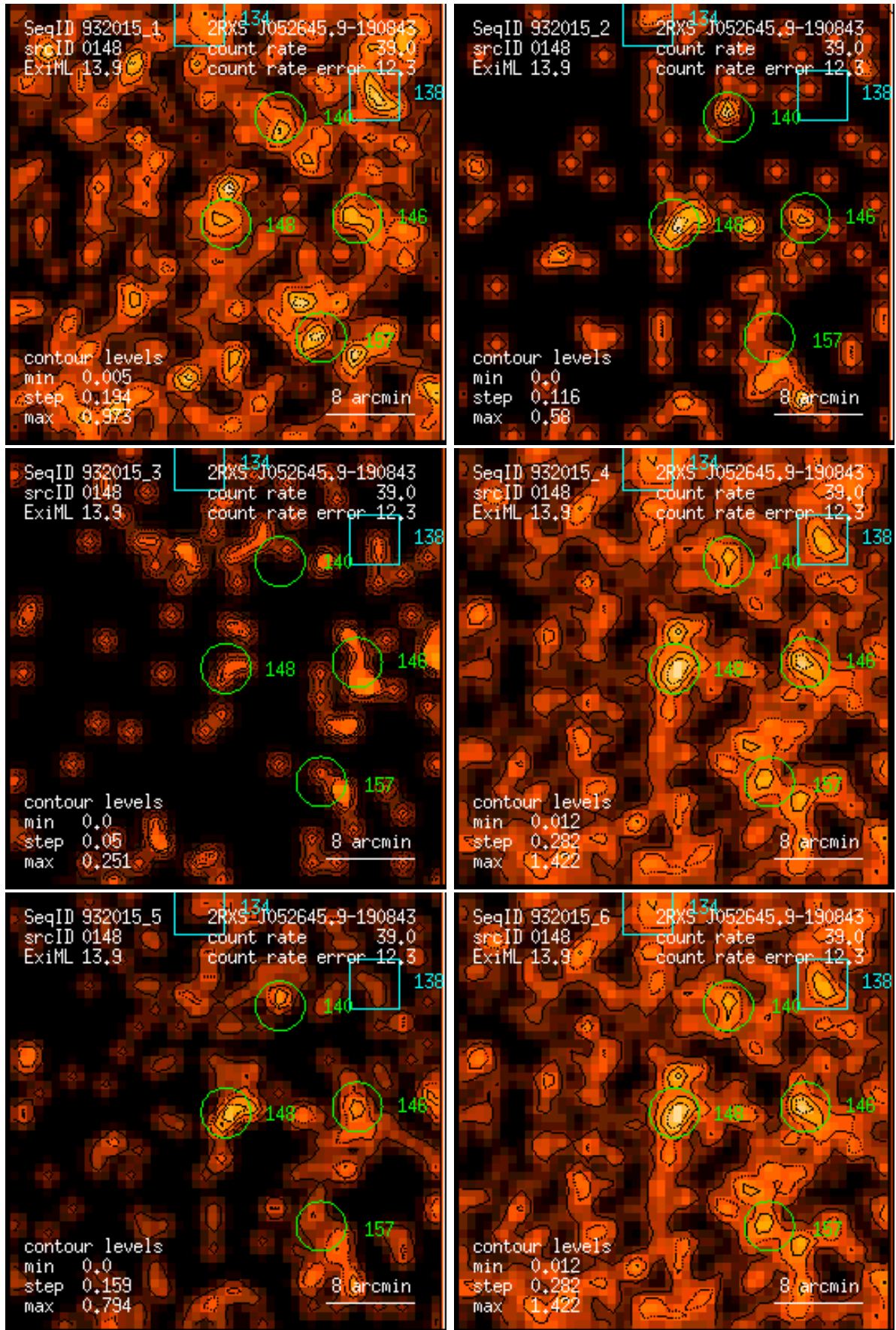
Figure 148: RASS 932015: detection 0148: band rate images, Gaussian filter: (1) PSPC channels 11 – 41, (2) 52 – 90, (3) 91 – 201, (4) 11 – 235, (5) 52 – 201, (6) 11 – 201. Broad band rates in counts/ks. Band rate contour levels in counts/ks/arcmin 2 .
