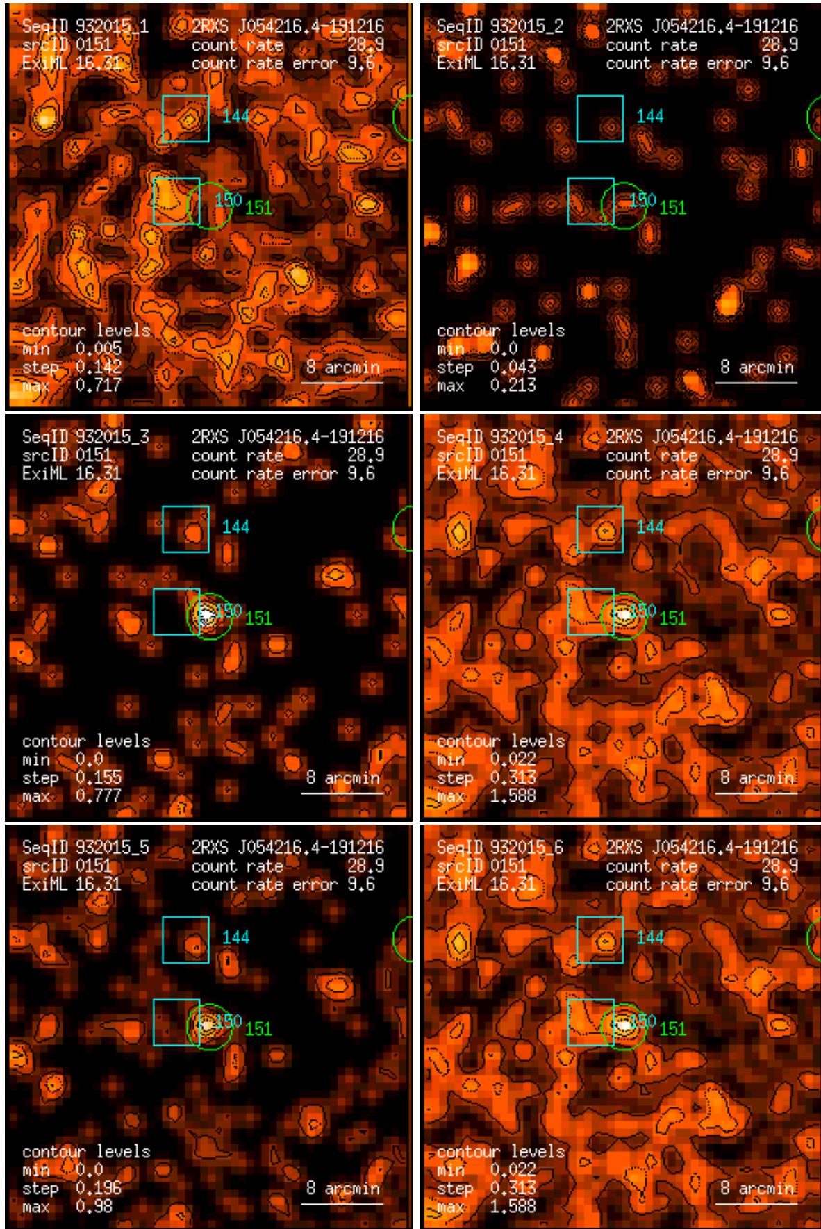
Figure 151: RASS 932015: detection 0151: band rate images, Gaussian filter: (1) PSPC channels 11 – 41, (2) 52 – 90, (3) 91 – 201, (4) 11 – 235, (5) 52 – 201, (6) 11 – 201. Broad band rates in counts/ks. Band rate contour levels in counts/ks/arcmin 2 .
