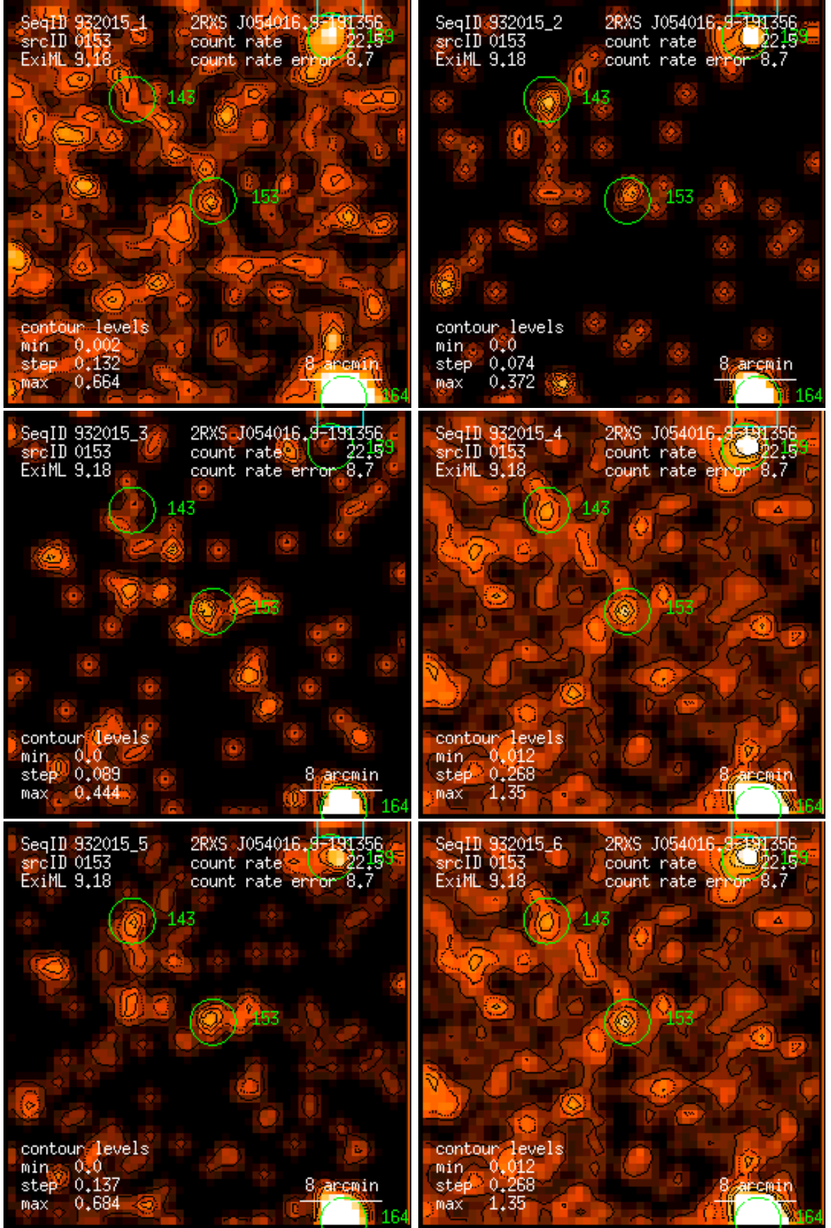
Figure 153: RASS 932015: detection 0153: band rate images, Gaussian filter: (1) PSPC channels 11 – 41, (2) 52 – 90, (3) 91 – 201, (4) 11 – 235, (5) 52 – 201, (6) 11 – 201. Broad band rates in counts/ks. Band rate contour levels in counts/ks/arcmin 2 .
