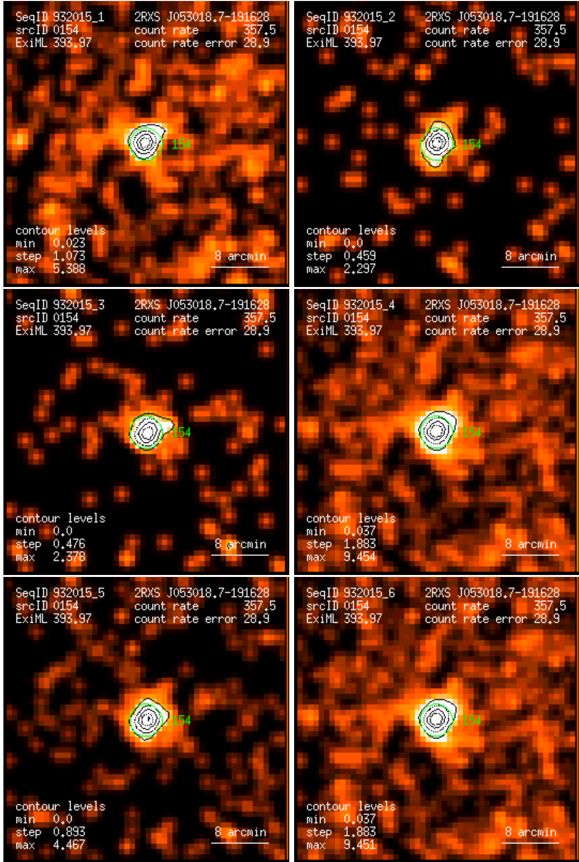
Figure 154: RASS 932015: detection 0154: band rate images, Gaussian filter: (1) PSPC channels 11 – 41, (2) 52 – 90, (3) 91 – 201, (4) 11 – 235, (5) 52 – 201, (6) 11 – 201. Broad band rates in counts/ks. Band rate contour levels in counts/ks/arcmin 2 .
